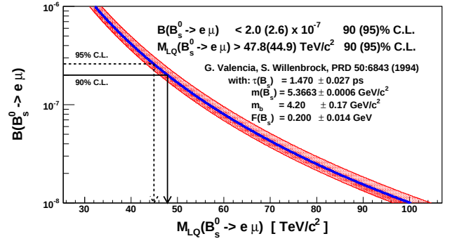
FIG. 3: Leptoquark mass limit corresponding to the 90 (95) % C.L. on \mathcal{B}(B_s^0 \rightarrow e^+\mu^-) . The error band is obtained by varying the values entering the theoretical calculation within their uncertainties. The uncertainties stemming from approximating \alpha_s are not included.
