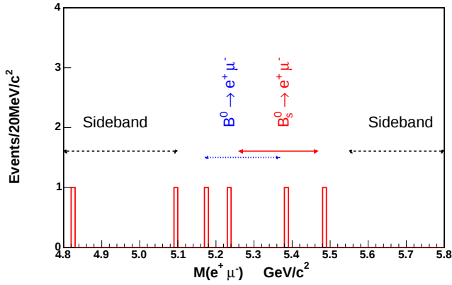
FIG. 1: Invariant mass distribution of e^+\mu^- pairs for events where one track passed the electron identification and the other track the muon identification. The B_s^0 ( B^0 ) search window is indicated by the solid (dotted) line. The sideband regions are indicated by the dashed lines.
