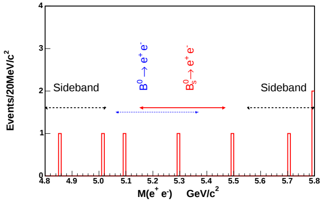
FIG. 2: Invariant mass distributions of e^+e^- pairs for events where both tracks passed the electron identification. The B_s^0 ( B^0 ) search window is indicated by the solid (dotted) line. The sideband regions are indicated by dashed lines.
