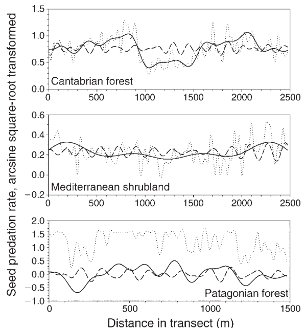
FIG. 4. Seed predation rate in the different study systems, along 2500-m (1500-m in the Patagonian forest) sampling transects. The arcsine square-root-transformed (and smoothing-spline-fitted) raw values (dotted line) and the values predicted by the principal coordinates of neighbor matrices (PCNM)-based spatial submodels at different spatial scales (broad, solid line; intermediate, dashed line) are distinguished. Seed predation rate was measured as the proportion of consumed seeds per plot.
