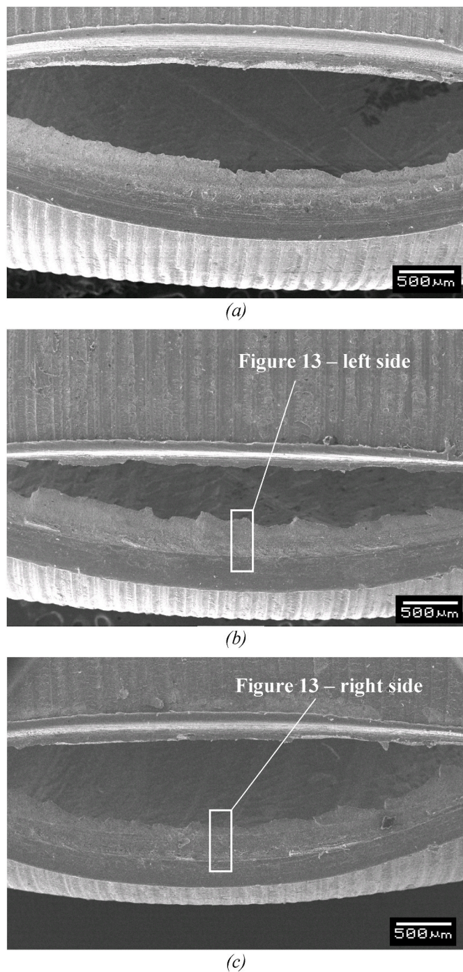
Fig. 12. General fracture surfaces. (a) Uncharged sample. (b) Hydrogen pre-charged and tested at 60 MPa/h in 1 M \text{H}_2\text{SO}_4 + 0.25 g/l \text{As}_2\text{O}_3 and (c) Hydrogen pre-charged and tested at 60 MPa/h in 3.5% NaCl. In Fig. 12(b) and (c) are indicated the areas analyzed at higher magnification in Fig. 13.
