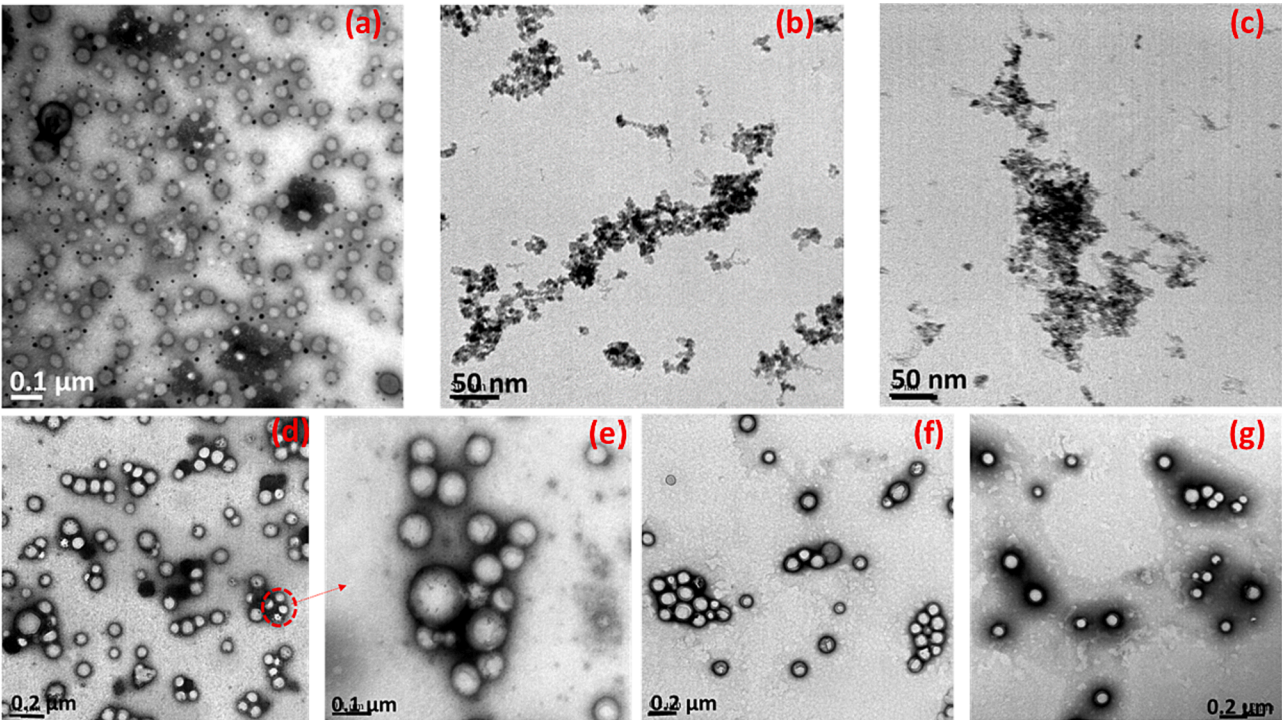
Fig. 3. TEM images of empty micelles (a), CeO 2 NPs A (b), CeO 2 NPs (c), PLGA micelles with the two formulations of CeO 2 NPs A (d) (e), and CeO 2 NPs B (f) (g).
