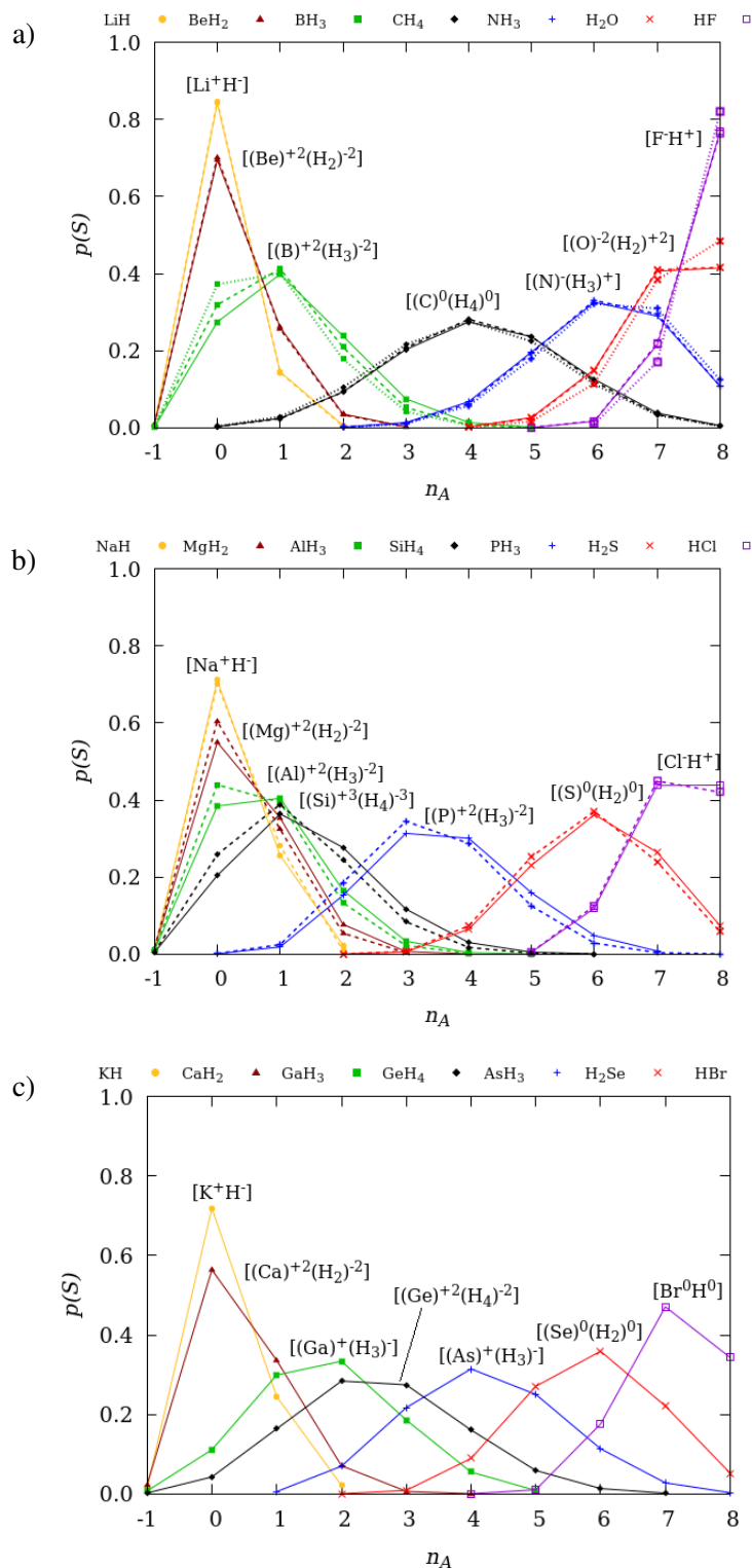
FIG. 2. 2-basin probabilities in the QTAIM framework for a) second-row, b) third-row, and c) fourth-row AH_n hydrides. B3LYP results are indicated in solid lines; CASSCF results are represented using dashed lines for a) and b); HF results are only displayed for a) using dotted lines. The most probable RSRs with B3LYP wave functions is given for each system. The meaning of n_A is explained in the text.
