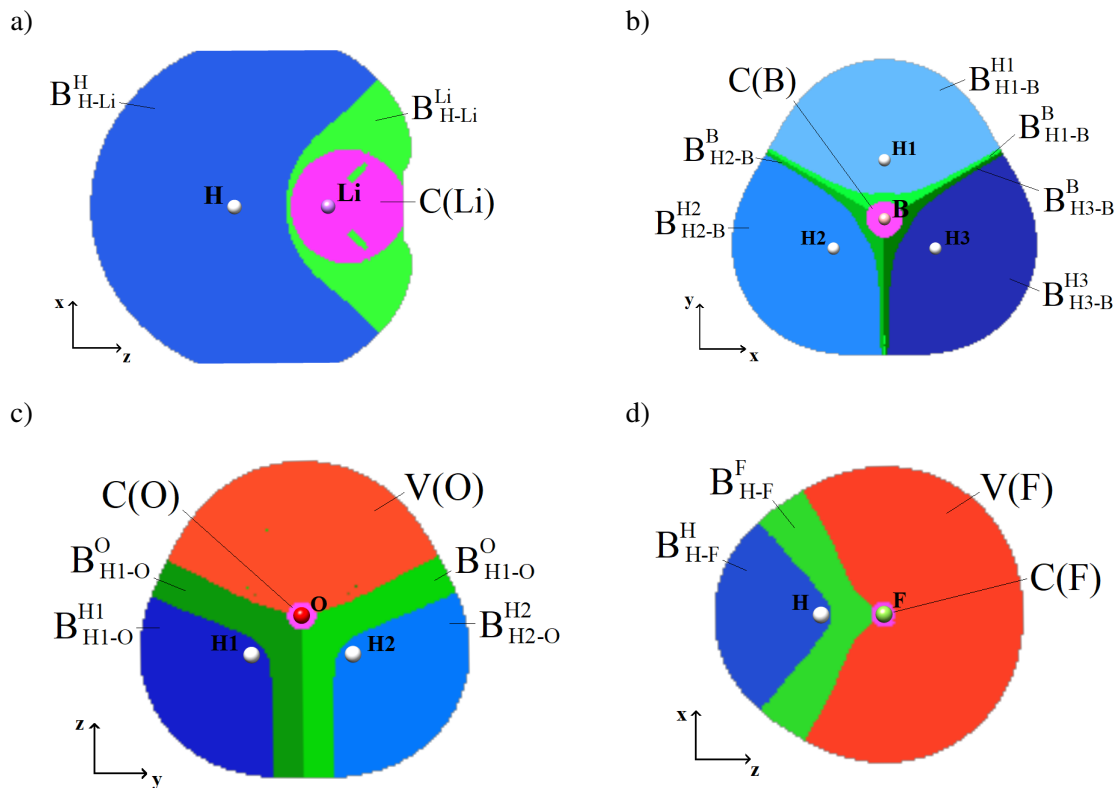
FIG. 3. ELFQAIM partitioning for a) LiH, b) BH 3 , c) H 2 O, d) HF projected on the \sigma_h plane. Bluish: hydrogen sub-region, B_{H-A}^H ; greenish: disynaptic bond sub-region, B_{H-A}^A ; pink: central atom core sub-region, C(A); orange: monosynaptic V(A) region. Note that different basins of the same type in the same molecule are coloured by using different color tones.
