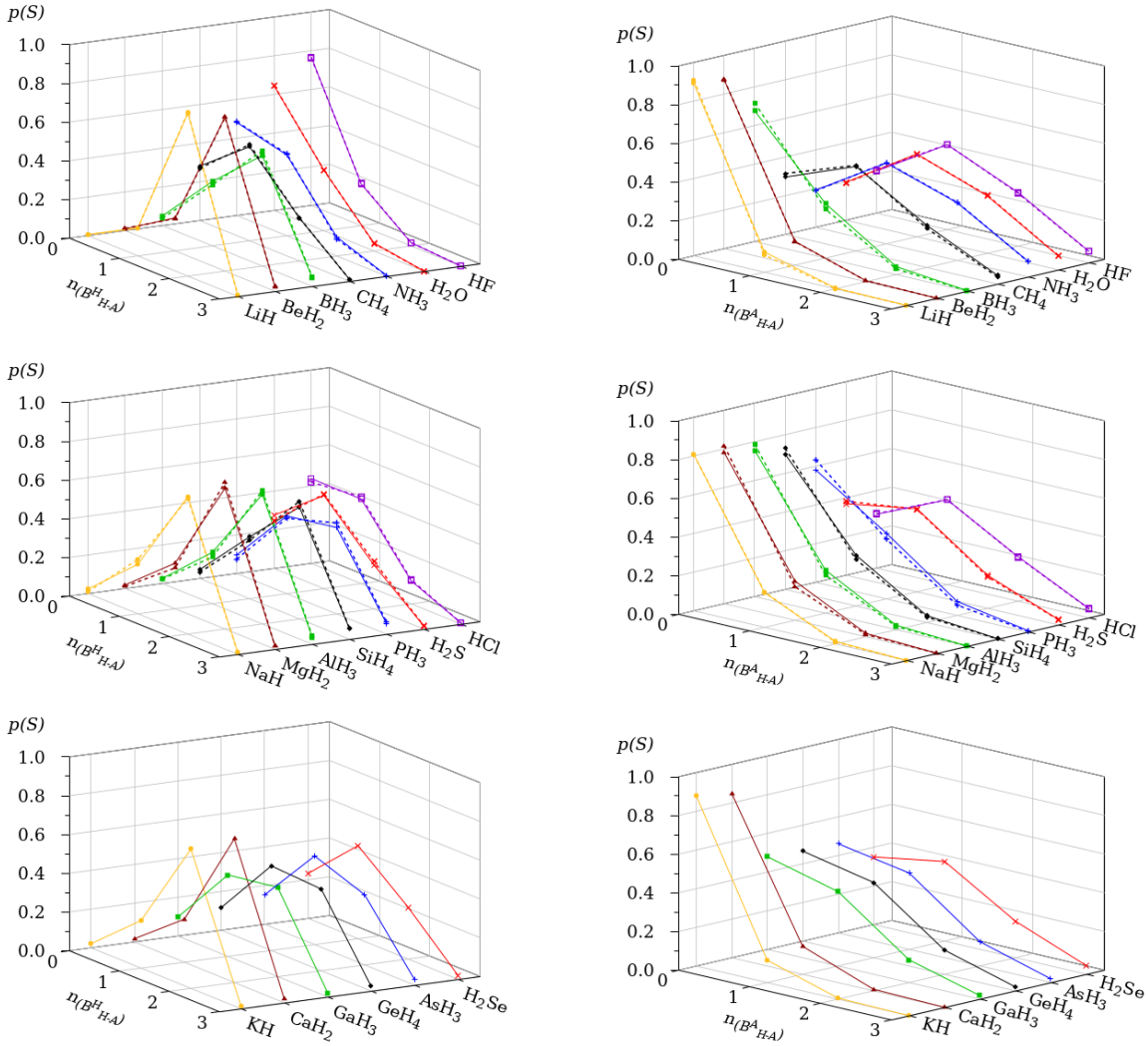
FIG. 4. 2- basin probabilities for hydrogen ( B_{H-A}^H ) (left) and bond ( B_{H-A}^A ) (right) sub-regions within QEI partition in second-row (top), third-row (middle) and fourth-row (bottom) AH_n hydrides. Solid lines: B3LYP wave function; dashed lines: CASSCF calculations.
