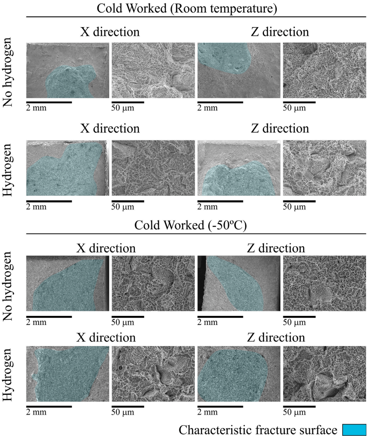
Fig. B.5. Fractographs of the tensile surfaces of the CW material after being tested.
