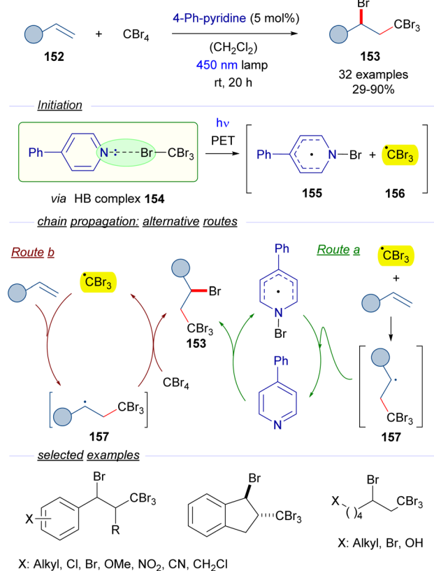
Scheme 24 ATRA reaction of olefins through the formation of a HB complex 154 with catalytic amounts of 4-phenylpyridine.
