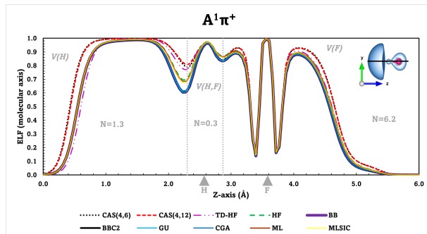
FIG. 2. Profile of the electron localization function (ELF) along the internuclear axis in the first excited state ( A^1\Pi^+ ) of the HF molecule as computed with CASSCF and several reconstructions of the 2-PDM at the TD-DFT level (see Table I). The inset shows the line along which the ELF has been plotted as well as an ELF isosurface with an iso-value of 0.83. F and H are depicted as red and light-gray points, respectively. The positions of F and H are marked with light-gray triangles. Vertical dashed lines indicate the location of the separatrices between the basins.
