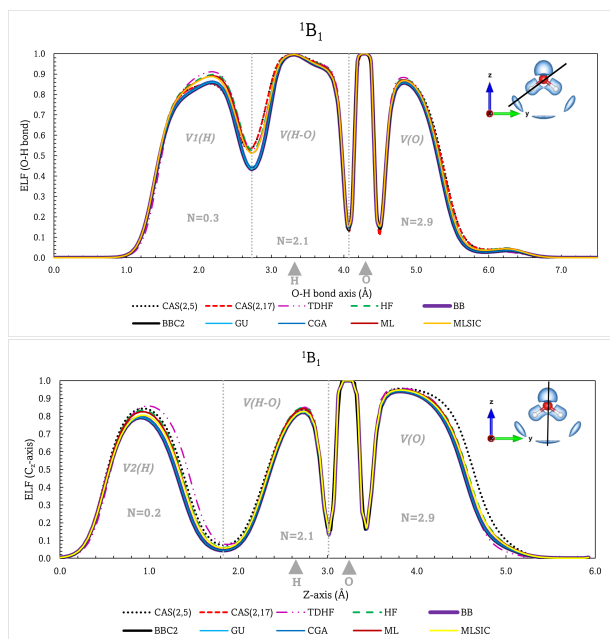
FIG. 6. Profile of the electron localization function (ELF) along the O-H bond axis (up) and in the C_2 axis (down) of the first excited state ( ^1B_1 ) of the water molecule. The insets show the lines along which the ELF has been plotted and a ELF = 0.83 isosurface. O and H are depicted as red and light-gray points in the inset, and with light-gray triangles in the profiles. Vertical dashed lines indicate the position of the separatrices between basins.
