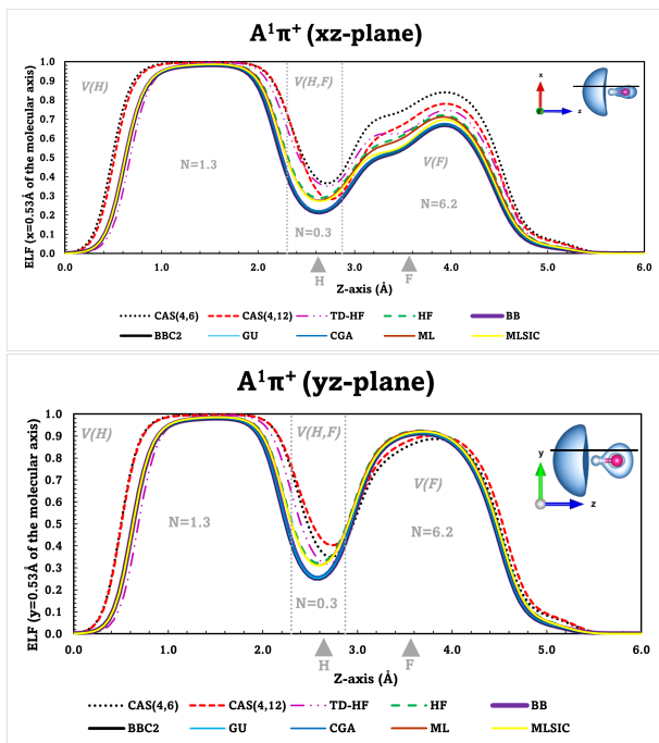
FIG. 3. Profiles of the electron localization function (ELF) computed 1 au ( 0.53\text{\AA} ) away from the internuclear axis in the first excited state ( A^1\Pi^+ ) of the hydrogen fluoride molecule as computed with CASSCF and several reconstructions of the 2 particle-reduced-density-matrix (see Table I). The up/down plots correspond to the ELF in the xz and yz planes, respectively. The insets show the line along which the ELF has been plotted and a ELF=0.83 isosurface, with F and H being depicted as red and light-gray points. The positions of F and H are marked with light-gray triangles. Vertical dashed lines indicate the location of the separatrices between the basins.
