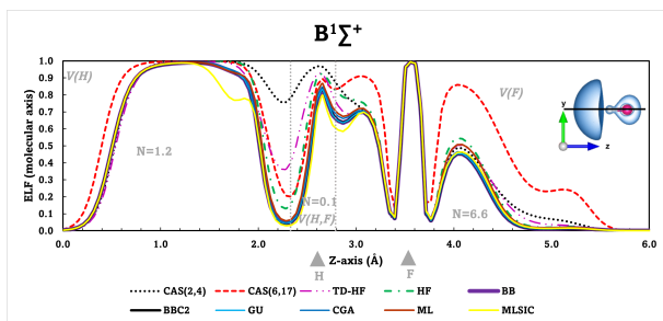
FIG. 4. Profile of the electron localization function (ELF) along the internuclear axis in the Franck-Condon geometry of the second excited state, B^1\Sigma^+ , of the hydrogen fluoride molecule, as computed with CASSCF and several reconstructions of the 2 particle-reduced-density-matrix (see Table I). The inset shows the line along which the ELF has been plotted and a ELF=0.77 isosurface. F and H are depicted as red and light-gray points in the inset. Positions of F and H are marked with light-gray triangles. Vertical dashed lines indicate the position of the separatrices between the ELF basins.
