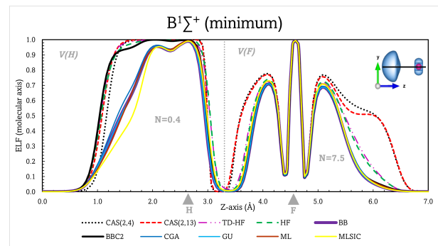
FIG. 5. Profile of the electron localization function (ELF) along the internuclear axis at the equilibrium distance of the second excited state, B^1\Sigma^+ , of the hydrogen fluoride molecule, as computed with CASSCF and several reconstructions of the 2 particle-reduced-density-matrix (see Table I). The inset shows the line along which the ELF has been plotted and a ELF=0.77 isosurface. F and H are depicted as red and light-gray points in the inset. Positions of F and H are marked with light-gray triangles. Vertical dashed lines indicate the position of the separatrices between the ELF basins.
