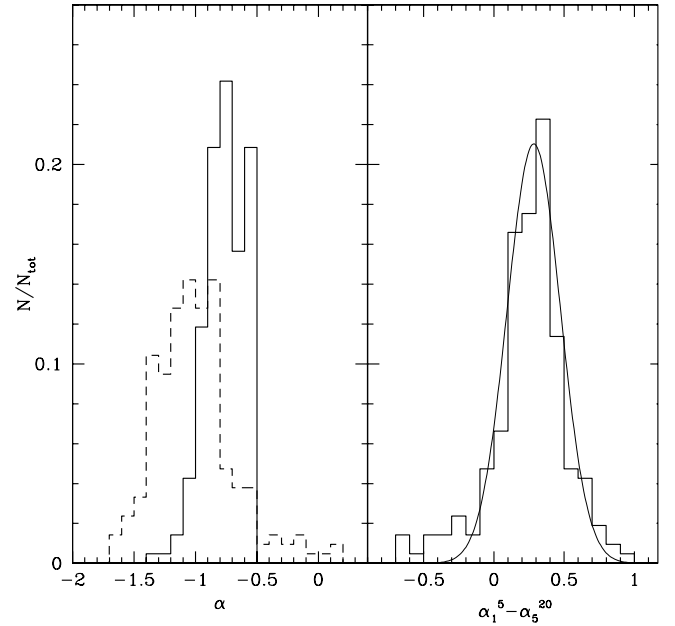
Fig. 4. Left panel: distributions of 1–5 GHz (solid line) and 5–20 GHz (dashed line) spectral indices of steep-spectrum sources selected from the AT20G catalogue. Right panel: distribution of the difference \alpha_1^5 - \alpha_5^{20} . The thin line is the Gaussian fit.
