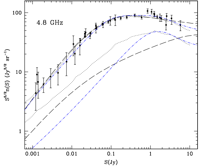
Fig. 1. Differential number counts normalized to S^{5/2} for ERS at 4.8 GHz. Filled squares are observational data (see De Zotti et al. 2010). The plotted curves represent the estimated number counts from the models by Toffolatti et al. (1998, dotted line), De Zotti et al. (2005, blue dash-dotted line), and Massardi et al. (2010, dashed line). Lower curves with the same line types as above represent the estimated number counts of flat-spectrum sources given by the same models.
