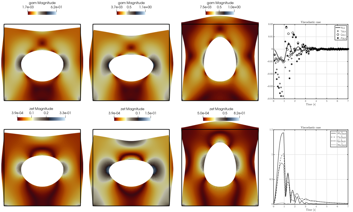
Figure 6.2: Example 2. Snapshots at 10x displacement magnification taken at times 0.5 s, 1 s, 1.5 s (left and two middle columns, respectively) of elastic and viscoelastic stresses for a viscoelastic material (top and bottom row, respectively). Solutions were obtained with a second order method. Right column plots: transients of vertical displacement and yy -components of elastic and viscous stresses at the point (0.5, 0.82) , as well as L^2 -norms of all quantities.
