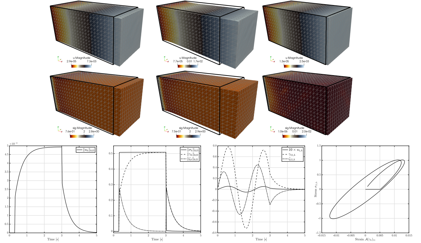
Figure 6.3: Example 3. Snapshots at 10x displacement magnification taken at times 0.33s, 3s, 3.6s (left, middle, right) of displacement (top) and distribution of total stress (middle row) for the creep of a viscoelastic slab. Solutions obtained with k = 1 . Bottom left: transients of L^2 -norms of displacement, and elastic, viscous, and total stresses for the case of creep. Bottom right: transients at the point (0.5, 0.25, 0.25) of x -displacement (magnified) and xx -stresses; and stress-strain curve for the cyclic loading case.
