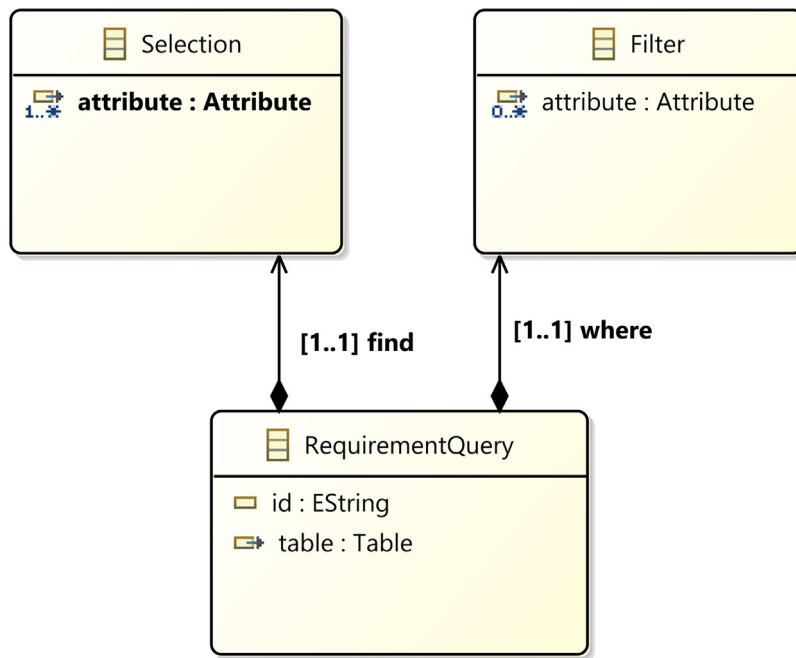
Fig. 3. Metamodel of the queries.
