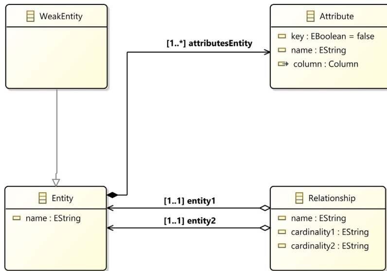
Fig. 2. Metamodel of the conceptual model.
