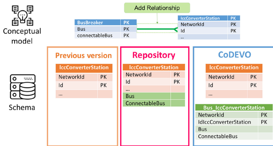
Fig. 8. CoDEvo schema vs repository schema of Type II version from project PowSybl for inserting a new relationship between entities BusBreaker and IccConverterStation. Orange: Table in previous version. Green: New table or columns for adding a relationship. (For interpretation of the references to color in this figure legend, the reader is referred to the web version of this article.)
