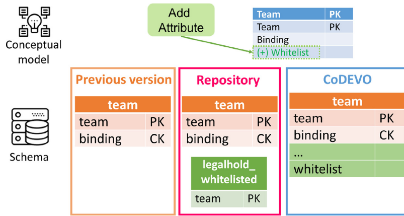
Fig. 7. Comparison between the CoDEvo schema and repository schema from the project WireApp for the addition of a boolean attribute “whitelist; to entity ‘Team’. Orange: Table in previous version. Green: New table or column for adding the attribute. (For interpretation of the references to color in this figure legend, the reader is referred to the web version of this article.)
