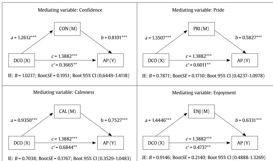
Figure 3. Diagrams and Results of the Simple Mediation Analyses (Process Four) Using Positive Emotions.
