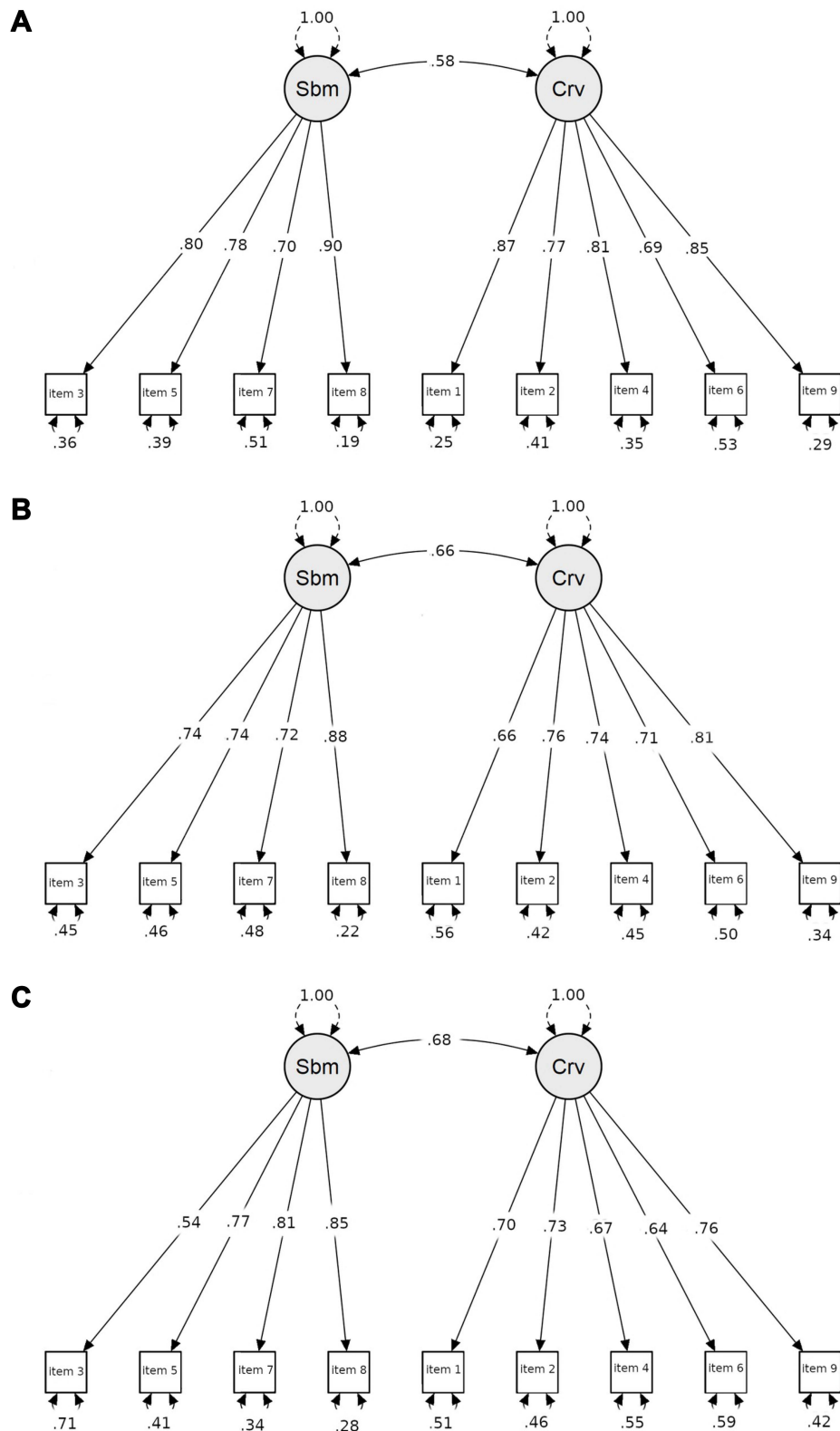
Figure 1 Standardized parameter estimates for the multigroup configural measurement model of the ADS-9. (A) clinical, (B) comparison, and (C) general population. All p < 0.001 .
