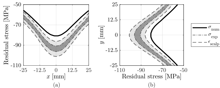
Fig. 15. Residual stress distribution on symmetrically tempered glass samples at H/D = 40 along (a) x direction and (b) y direction.
