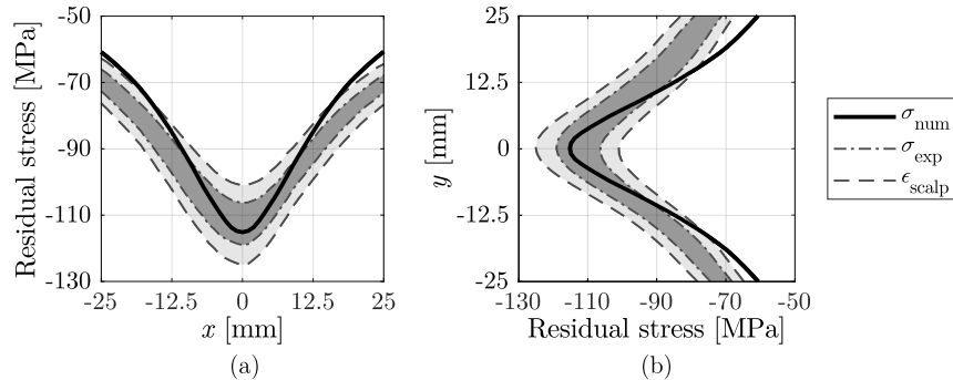
Fig. 14. Residual stress distribution on symmetrically tempered glass samples at H/D = 20 along (a) x direction and (b) y direction.
