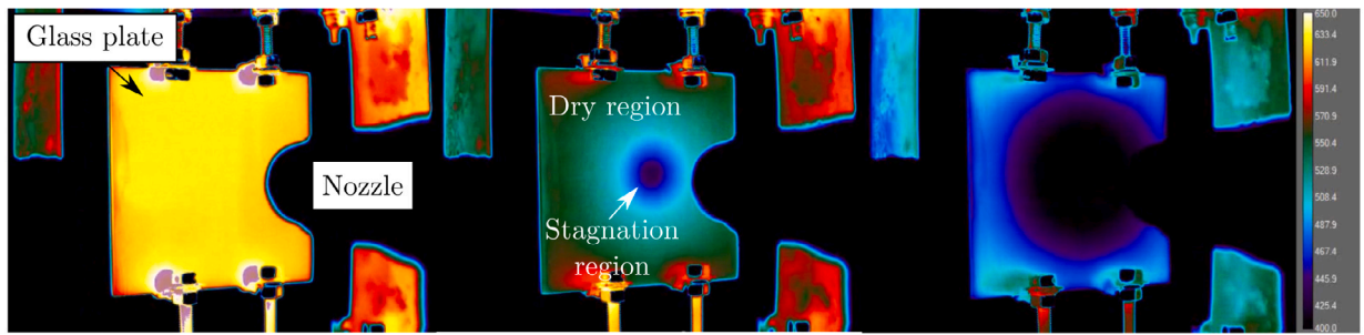
Fig. 7. Temperature distribution on the glass surface recorded by thermography during the cooling down process.
