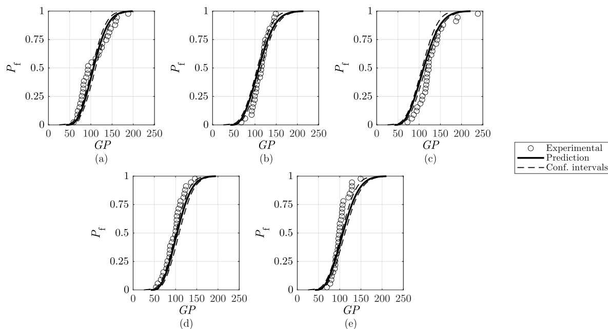
Fig. 25. Joint evaluation based on the merging of all the experimental tests to predict the failure probability of (a) AA, (b) STHD20, (c) STHD40, (d) ATHD20 and (e) ATHD40.
