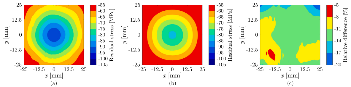
Fig. 11. Residual stress distribution on the front surface of symmetrically tempered glass samples at H/D = 40 : (a) experimental average, (b) modified procedure and (c) deviation.
