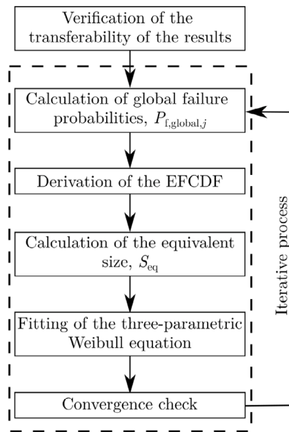
Fig. 6. Flowchart of the calculation sequence to fit the three-parametric Weibull distribution by the joint test evaluation.
