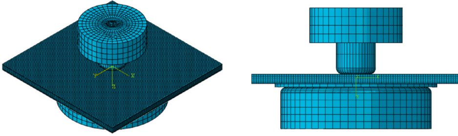
Fig. 4. Mesh of the in-service model composed of a load ring, support ring, silicon rubber and glass specimen.
