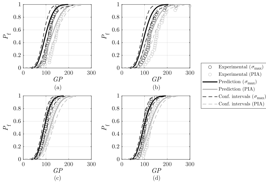
Fig. 24. Failure probability of tempered glass plates considering the PFCDF based on maximum principal stress and PIA failure criteria and derived from annealed glass experimental data: (a) STHD20, (b) STHD40, (c) ATHD20 and (d) ATHD40.
