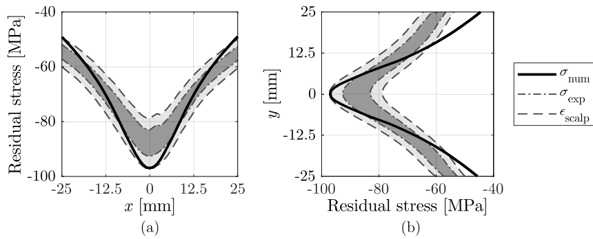
Fig. 16. Residual stress distribution on asymmetrically tempered glass samples for H/D = 20 along (a) x direction and (b) y direction.
