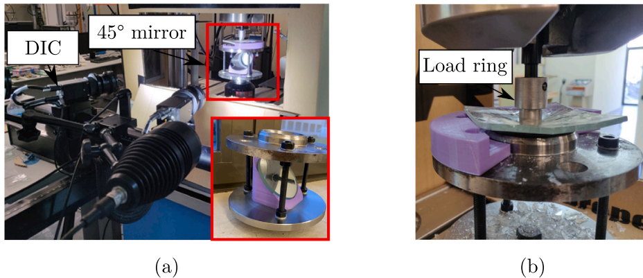
Fig. 8. Experimental CDR set-up: (a) ARAMIS 3D GOM equipment with an inclined mirror at 45°, and (b) CDR test until fracture of the specimen.
