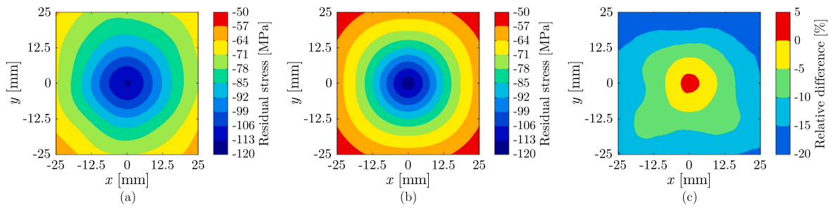
Fig. 10. Residual stress distribution on the front surface of symmetrically tempered glass samples at H/D = 20 : (a) experimental average, (b) modified procedure and (c) deviation.
