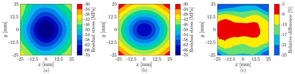
Fig. 13. Residual stress distribution on the front surface of asymmetrically tempered glass samples at H/D = 40 : (a) experimental average, (b) modified procedure and (c) deviation.
