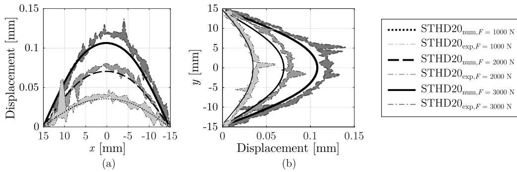
Fig. 19. Comparison between experimental and numerical displacement paths of symmetrically tempered glass samples for H/D = 20 along (a) x direction and (b) y direction.
