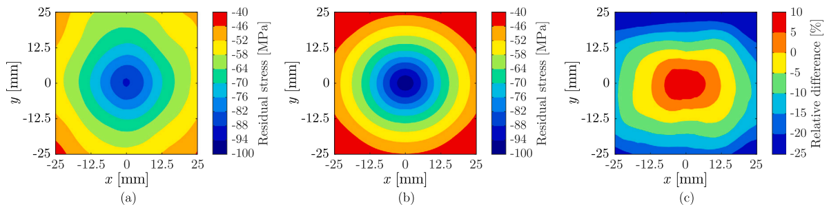
Fig. 12. Residual stress distribution on the front surface of asymmetrically tempered glass samples at H/D = 20 : (a) experimental average, (b) modified procedure and (c) deviation.
