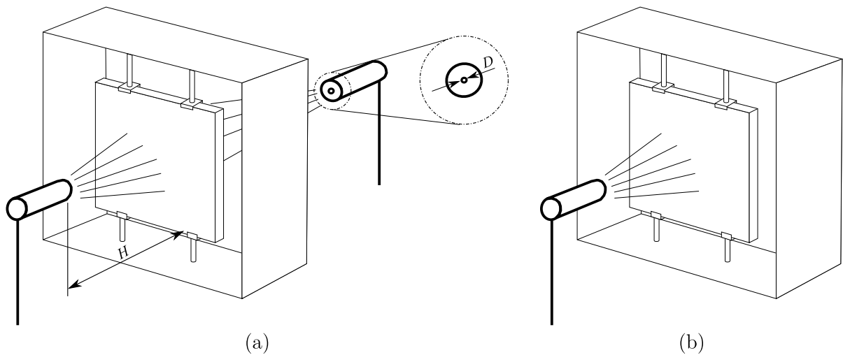
Fig. 1. Cooling down unit of (a) symmetrically tempered glass plates and (b) asymmetrically tempered glass plates.
