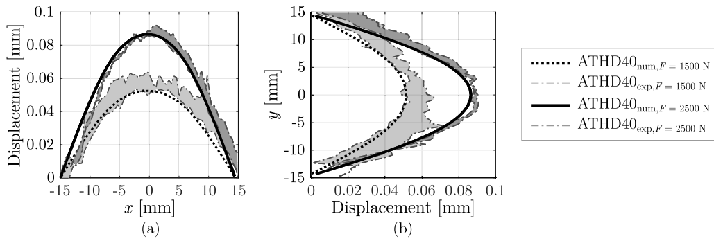
Fig. 22. Comparison between experimental and numerical displacement paths on asymmetrically tempered glass samples for H/D = 40 along (a) x and (b) y directions.
