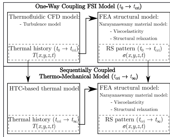
Fig. 3. Flow chart of the proposed procedure to estimate the residual stress pattern over time, where a one-way FSI approach is proposed until the critical temperature instant ( t_{crit} ) is attained and a sequentially coupled thermo-mechanical approach is proposed from t_{crit} to steady-state temperature instant ( t_{\infty} ). Reprinted from [39].
