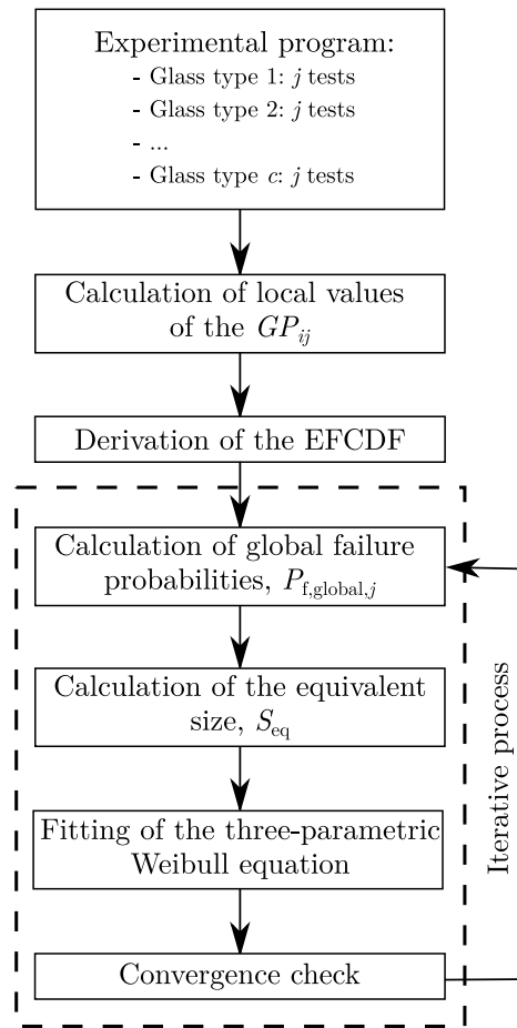
Fig. 5. Flowchart of the calculation sequence to fit the three-parametric Weibull distribution.
