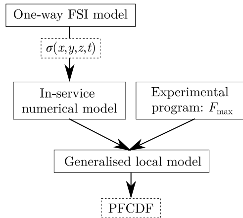
Fig. 2. Flow chart of the proposed numerical-statistical procedure to predict the probability of failure of pre-stressed structural glass components.
