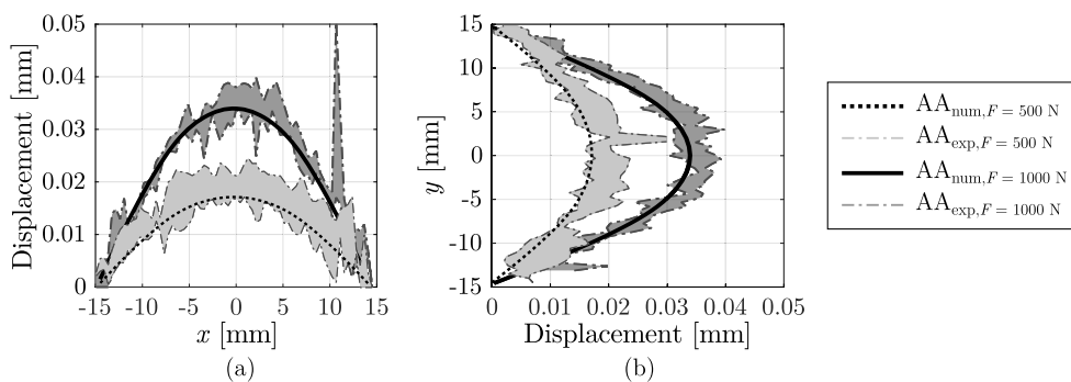
Fig. 18. Comparison between experimental and numerical displacement paths in annealed glass specimens along (a) x direction and (b) y direction.
