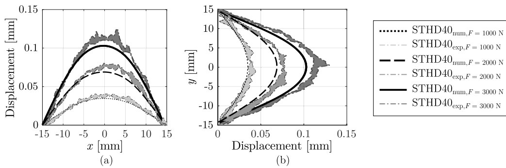
Fig. 20. Comparison between experimental and numerical displacement paths on symmetrically tempered glass samples for H/D = 40 along (a) x direction and (b) y direction.
