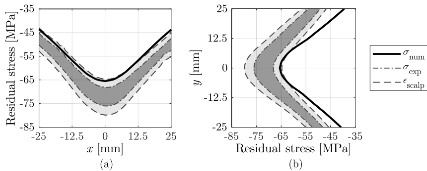
Fig. 17. Residual stress distribution on asymmetrically tempered glass samples for H/D = 40 along (a) x direction and (b) y direction.
