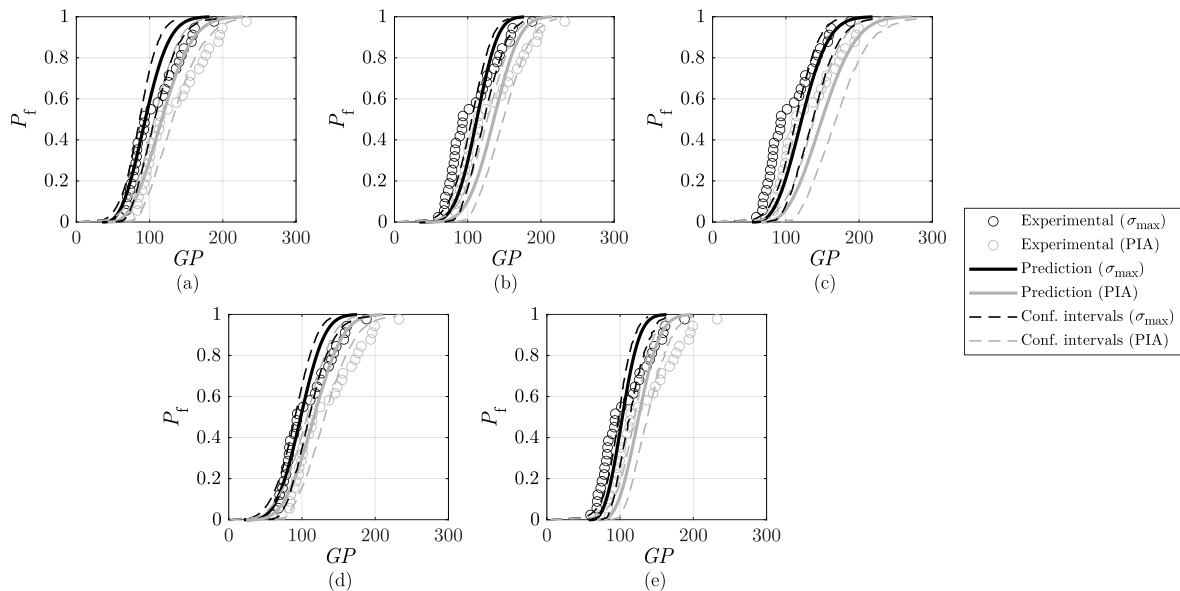
Fig. 23. Failure probability prediction of annealed glass plates considering the PFCDF based on maximum principal stress and PIA failure criteria and derived from (a) own experiments, (b) STHD20, (c) STHD40, (d) ATHD20 and (e) ATHD40.
