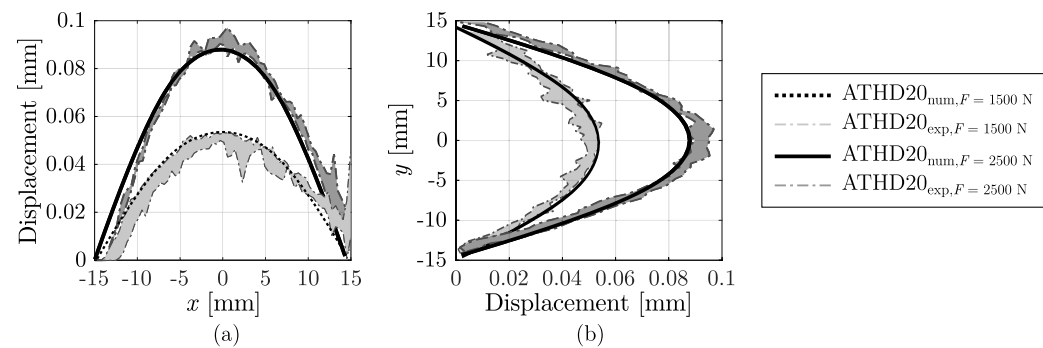
Fig. 21. Comparison between experimental and numerical displacement paths on asymmetrically tempered glass samples for H/D = 20 along (a) x and (b) y directions.
