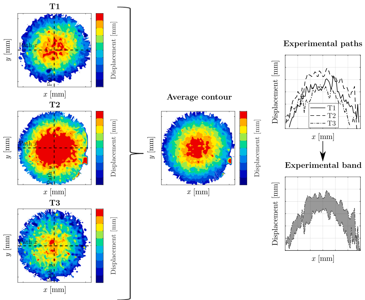
Fig. 9. Experimental post-processing procedure for the results of the CDR tests.
