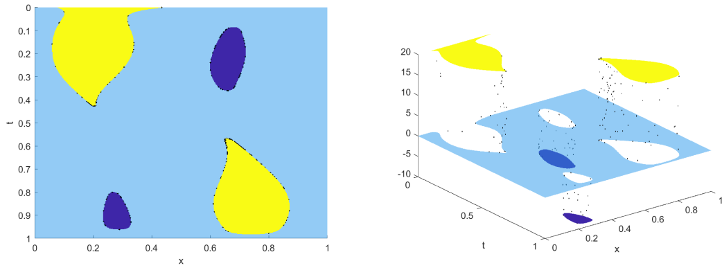
Figure 1: The optimal control exhibits a typical bang-off-bang behaviour. Black dots have been marked in the few space-time patches where the numerical approximation exhibits a singular behaviour.
