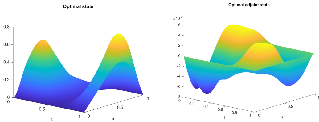
Figure 2: Optimal state and adjoint state.
