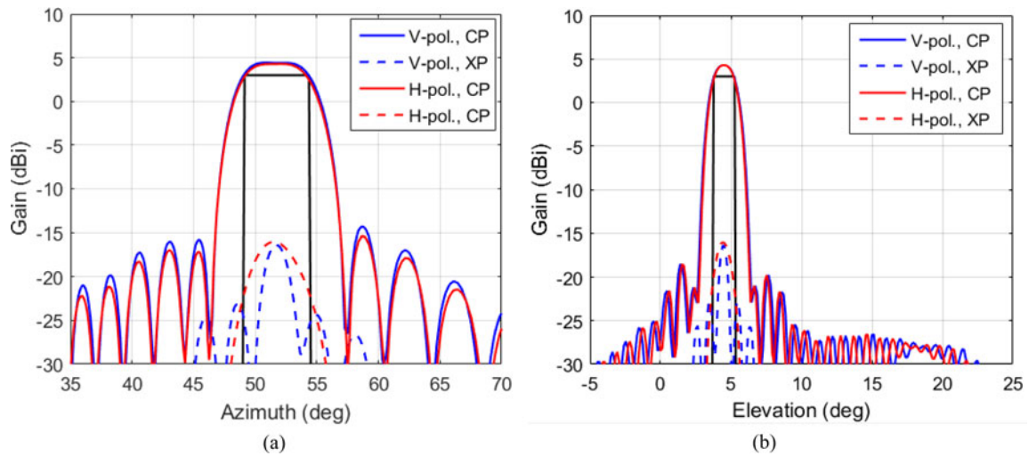
Fig. 13. KLONE 2: simulated radiation patterns at 27.7 GHz in the (a) azimuth and (b) elevation planes, including co-polar (CP) and cross-polar (XP) components.
