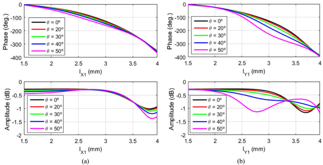
Fig. 3. Phase and amplitude responses of the reflectarray cell at 27.7 GHz for (a) V-polarization and (b) H-polarization under different incidence conditions: considering different values of \theta , while keeping constant the value of \varphi_i to 90^\circ .
