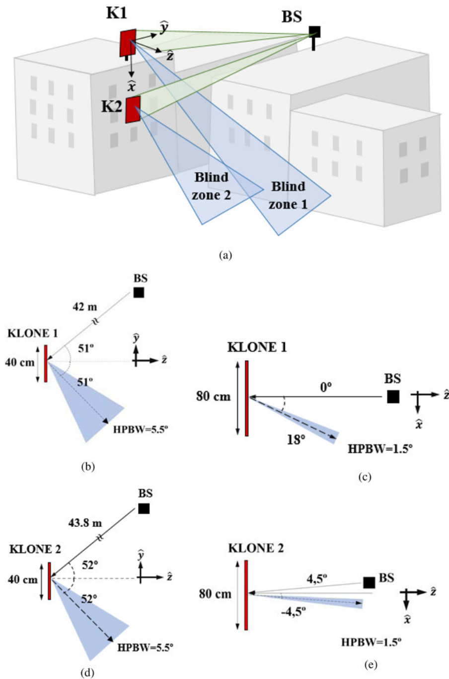
Fig. 1. (a) Outdoor scenario with two reflectarray panels (K1 and K2) installed on the wall and illuminated from a FR2 5G BS. (b, d) Azimuth view and (c, e) elevation view of the outdoor scenario for K1 (b, c) and K2 (d, e).
