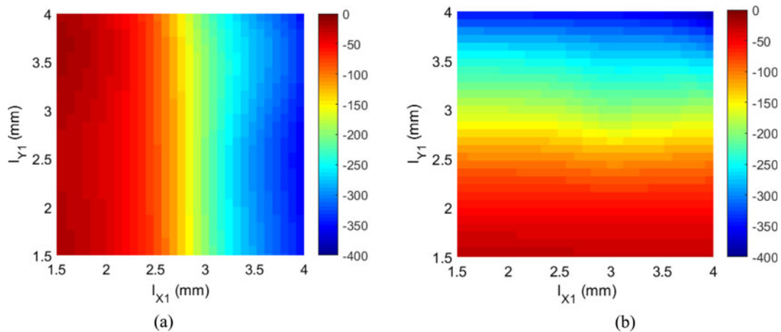
Fig. 4. Phase response (in degrees) of the reflectarray cell at 27.7 GHz, considering oblique incidence with \theta_i = 50^\circ , \varphi_i = 90^\circ : (a) V-polarization and (b) H-polarization.
