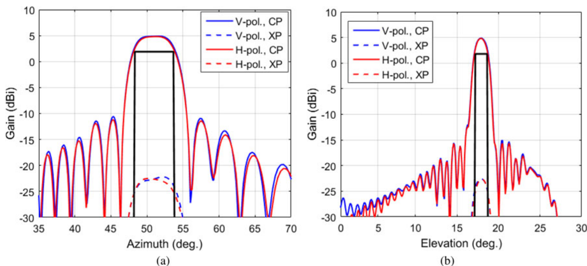
Fig. 12. KLONE 1: simulated radiation patterns at 27.7 GHz in the (a) azimuth and (b) elevation planes, including co-polar (CP) and cross-polar (XP) components.
