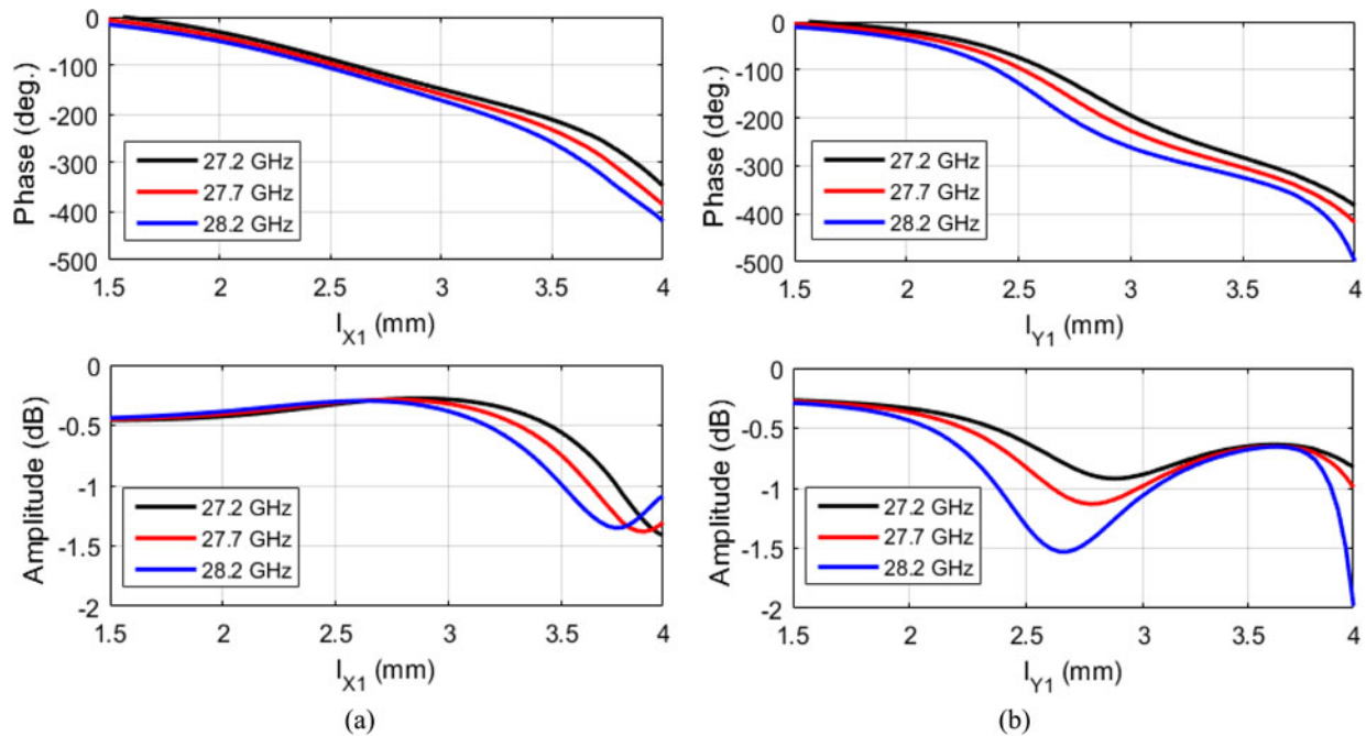
Fig. 5. Phase and amplitude responses of the reflectarray cell at different frequencies for (a) V-polarization and (b) H-polarization, considering oblique incidence with \theta_i = 50^\circ , \varphi_i = 90^\circ .
