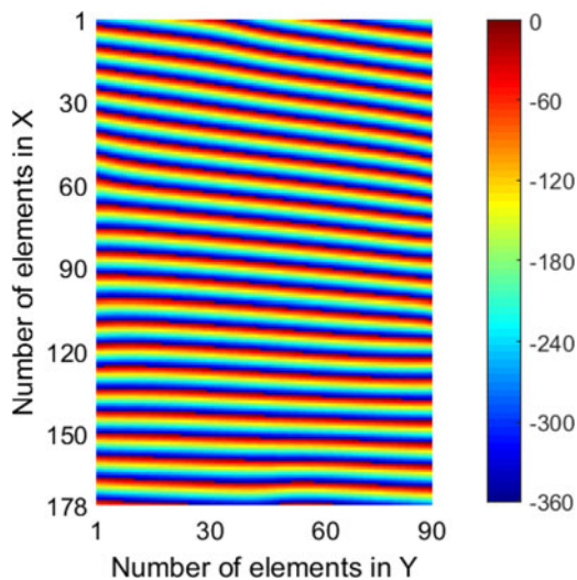
Fig. 10. Phase distribution (in degrees) after POS for K1.
