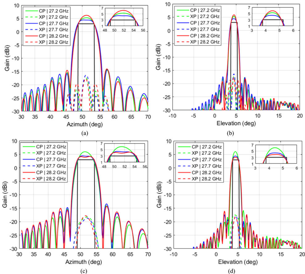
Fig. 15. KLONE 2: simulated co-polar (CP) and cross-polar (XP) radiation patterns at central and extreme frequencies: in V-polarization for the (a) azimuth and (b) elevation cuts, and in H-polarization for the (c) azimuth and (d) elevation cuts.
