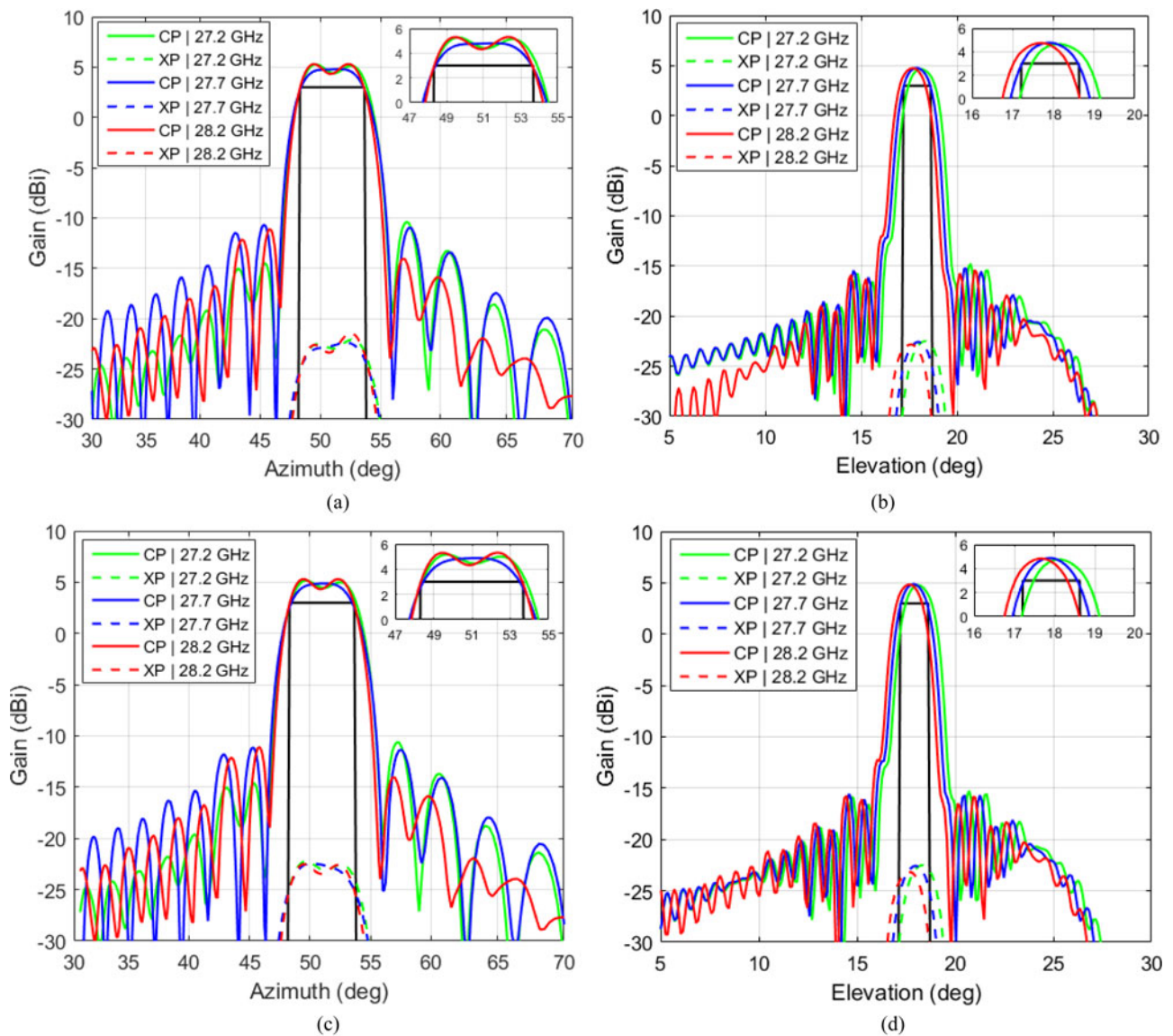
Fig. 14. KLONE 1: simulated co-polar (CP) and cross-polar (XP) radiation patterns at central and extreme frequencies: in V-polarization for the (a) azimuth and (b) elevation cuts, and in H-polarization for the (c) azimuth and (d) elevation cuts.
