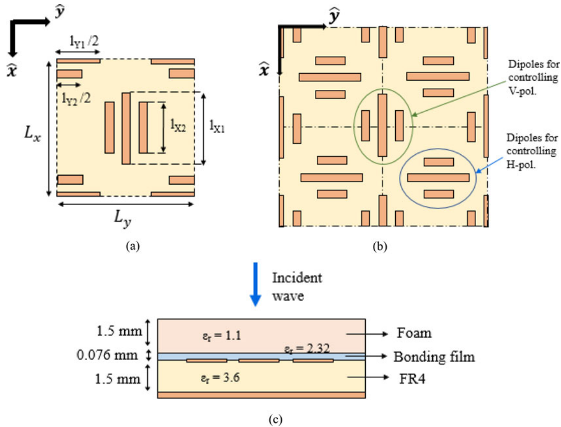
Fig. 2. Upper view of (a) the periodic unit cell and (b) the reflectarray periodic structure. (c) Lateral view with the stack-up configuration.
