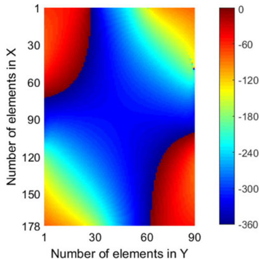
Fig. 11. Phase distribution (in degrees) after POS for K2.
