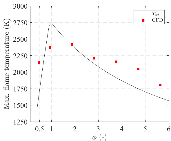
Fig. 13. Maximum flame temperature as function of equivalence ratio for Cupressus Funebri (biomass 2).
