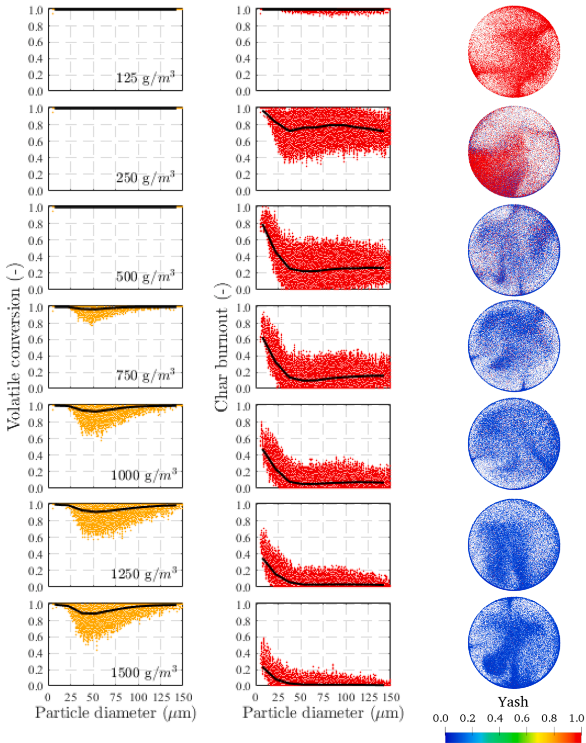
Fig. 15. Comparison of volatile conversion and char burnout as function of particle diameter for the various dust concentrations of Cupressus Funebris (biomass 2). Instantaneous data (dots) and profiles extracted by moving average (solid lines). On the right, particle tracks colored by ash fraction.
