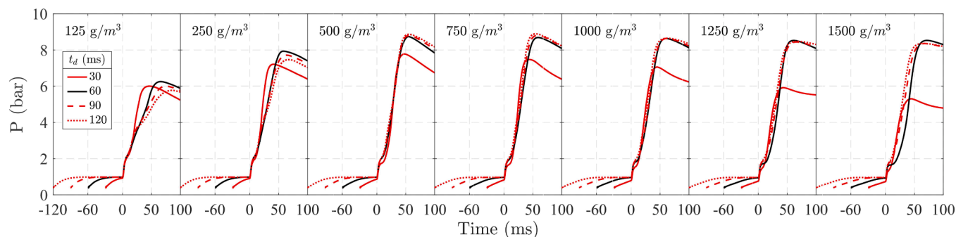
Fig. 25. Comparison of the different pressure-time curves obtained by varying the ignition delay time in the explosion process of Cupressus Funebriis (biomass 2).
