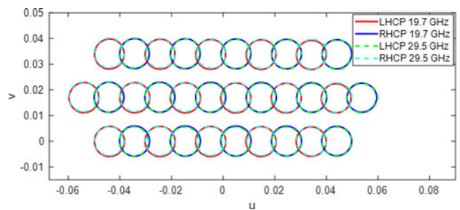
Fig. 11. Contour patterns of the 32 beams generated by 16 dual-CP feeds.
