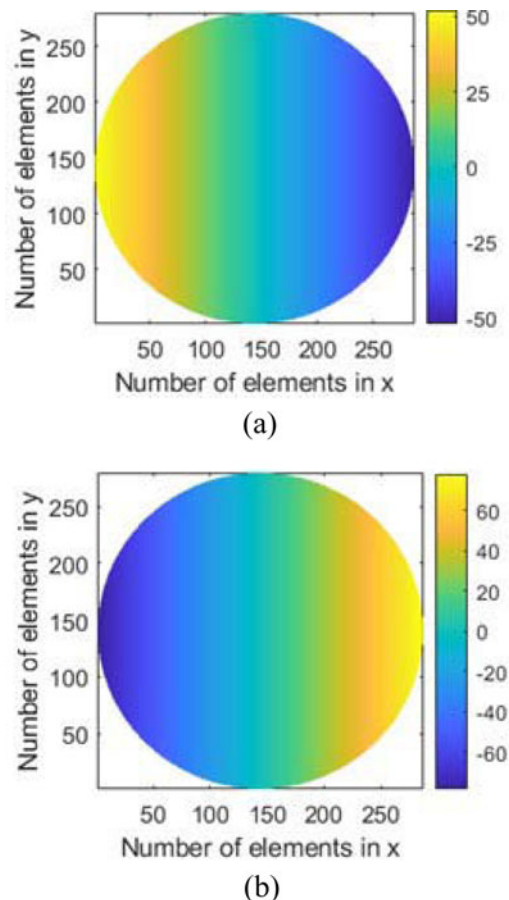
Fig. 8. Rotation angles (°) of (a) the arcs and (b) the dipoles.
