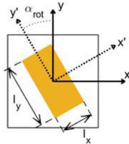
Fig. 1. Reflectarray cell based on a rectangular patch with a rotation angle \alpha_{rot} = 30^\circ .
