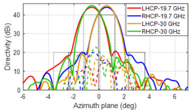
Fig. 18. Cut of the measured radiation patterns for the beams generated by one feed.
