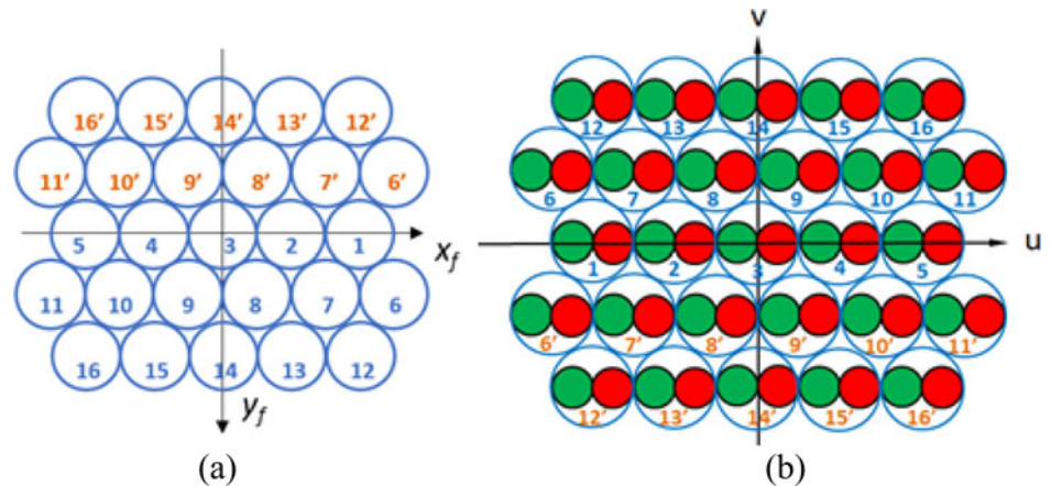
Fig. 10. Distribution of (a) the 27 feed-horns and (b) the 54 spots associated to the feeds.
