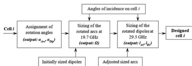
Fig. 9. Scheme of the cell design process.
