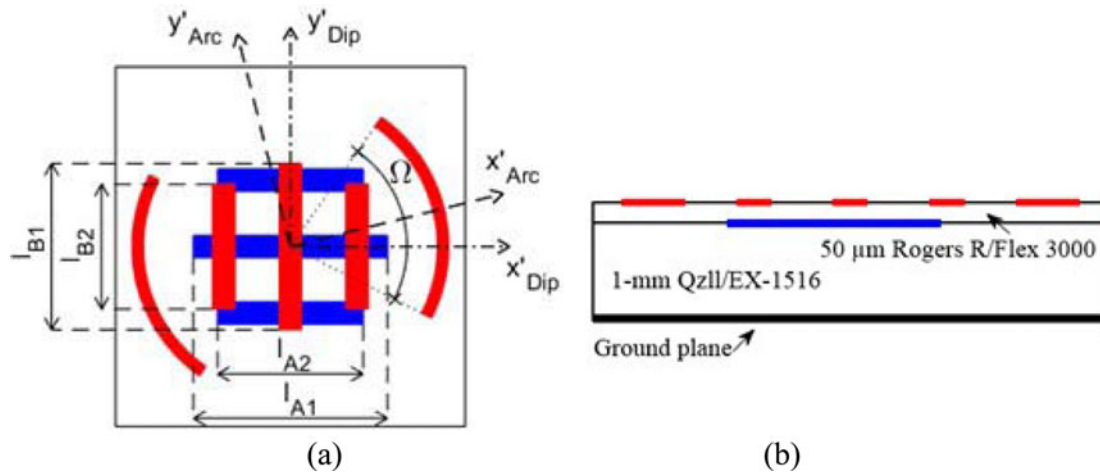
Fig. 3. Proposed reflectarray cell. (a) Top view, (b) lateral view.
