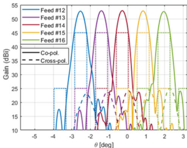
Fig. 15. Simulated radiation patterns in LHCP at 29.5 GHz in the plane \nu = 0.034 (generated by feeds 12-16).
