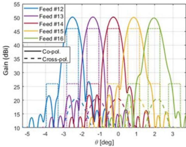
Fig. 13. Simulated radiation patterns in RHCP at 19.7 GHz in the plane \nu = 0.034 (generated by feeds 12-16).
