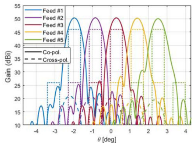
Fig. 12. Simulated radiation patterns in RHCP at 19.7 GHz in the plane v=0 (generated by feeds 1–5).
