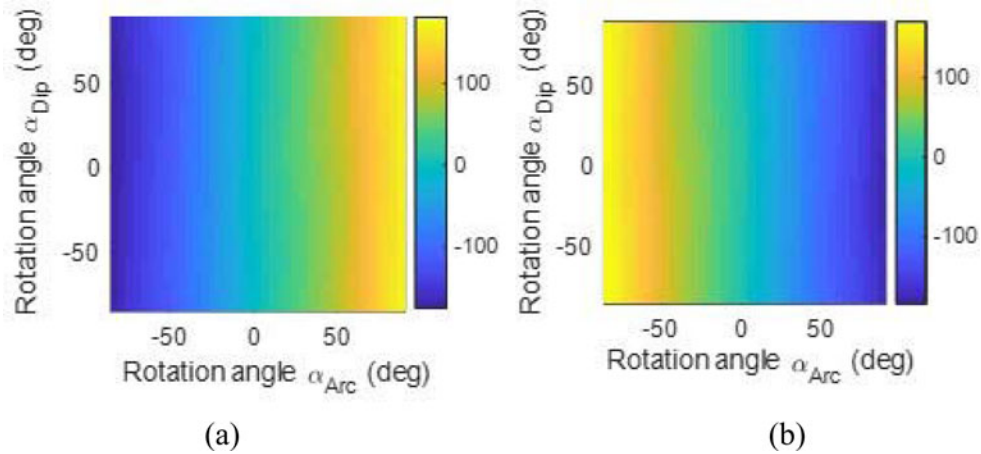
Fig. 4. Phase (°) in (a) RHCP and (b) LHCP introduced at 19.7 GHz when the arcs and dipoles are independently rotated.
