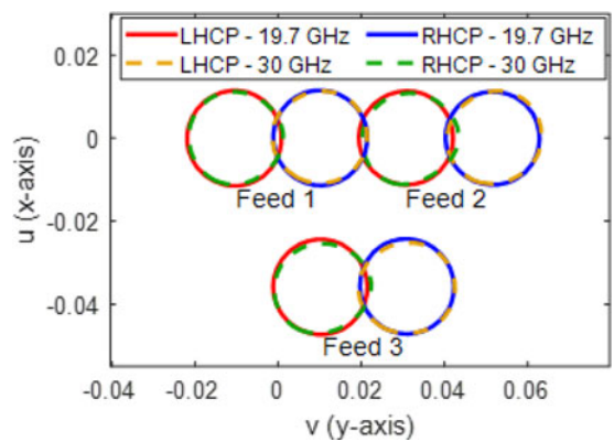
Fig. 17. Measured contour patterns at 40.6 dBi of the six beams generated by three feeds.
