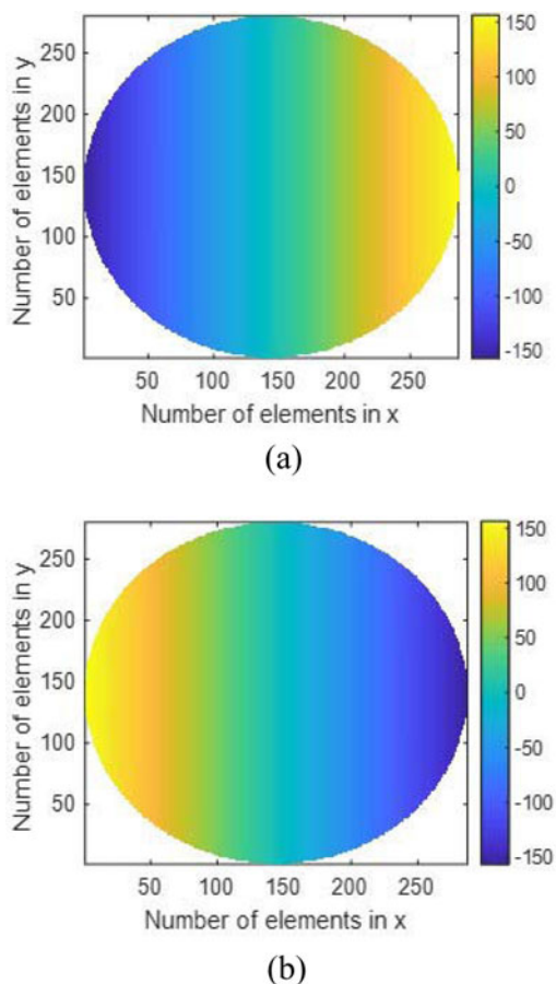
Fig. 7. Required phase distribution (°) at 29.5 GHz. (a) RHCP, (b) LHCP.
