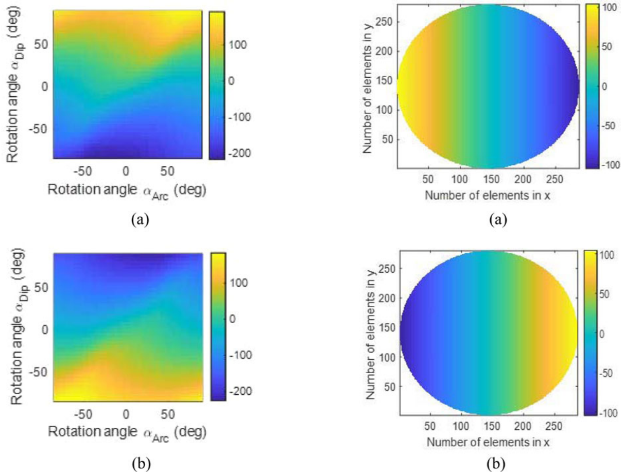
Fig. 5. Phase (°) in (a) RHCP and (b) LHCP introduced at 29.5 GHz when the arcs and dipoles are independently rotated.
