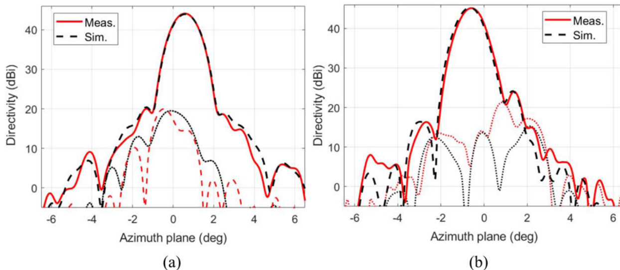
Fig. 19. Cut of the measured and simulated radiation patterns for the beam generated in RHCP by one feed at (a) 19.7 GHz and (b) 29.5 GHz.
