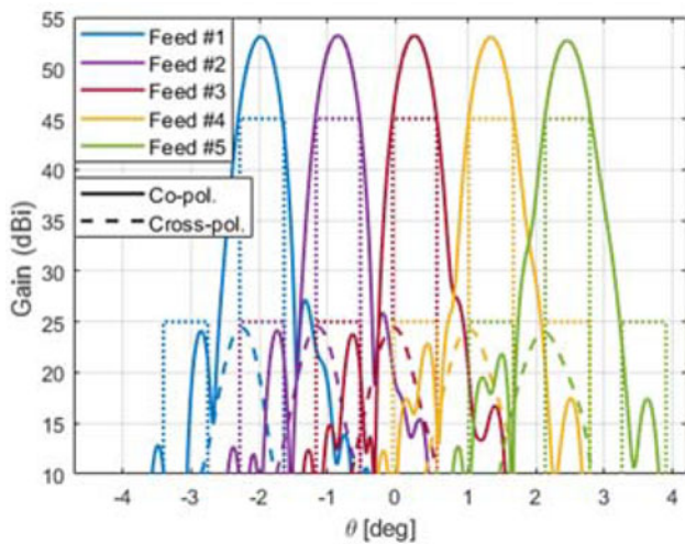
Fig. 14. Simulated radiation patterns in LHCP at 29.5 GHz in the plane \nu = 0 (generated by feeds 1-5).
