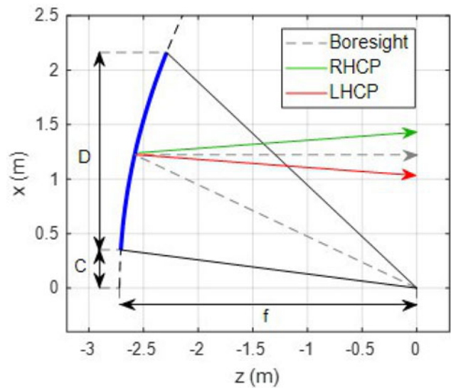
Fig. 2. Parabolic reflectarray antenna with the boresight and scanned directions of radiation.
