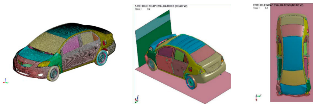
Fig. 2. NCAC's FE model for the 2010 Toyota Yaris Passenger Sedan and EuroNCAP full width frontal impact test simulation
