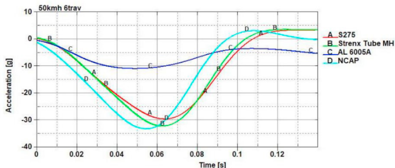
Fig. 7. Car deceleration (g's) for simulations at 50 km/h with different materials in the lateral protection systems: (A) S275; (B) Strenx 700 MH; (C) Aluminium 6005A-T6; (D) NCAP rigid wall
