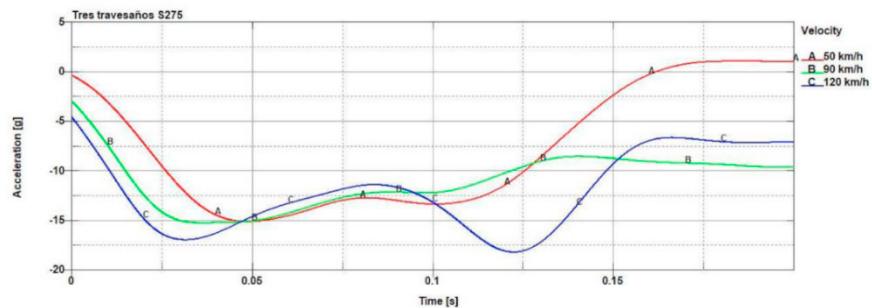
Fig. 9. Car deceleration (g's) for S275 three-post system: (A) 50 km/h; (B) 90 km/h; (C) 120 km/h
