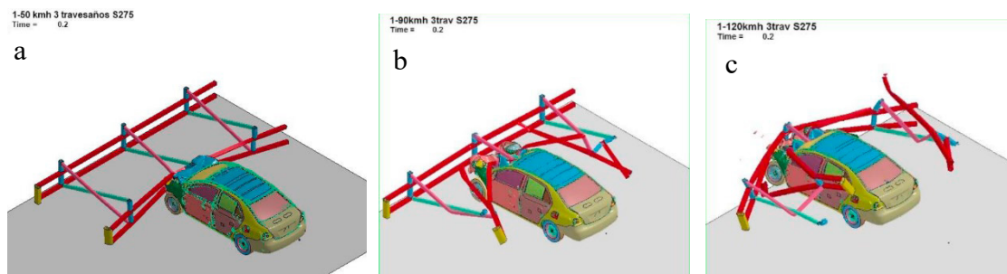
Fig. 8. Crash against S275 three-post system: (a) 50 km/h; (b) 90 km/h; (c) 120 km/h.
