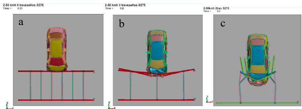
Fig. 4. Final frame for simulations at 50 km/h with S275 lateral protection systems: (a) Six-post system; (b) Three-post system; (c) Two-post system
