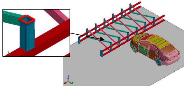
Fig. 3. Numerical model simulating a collision against the six-post lateral protection system. Constrained nodes at the top of the posts
