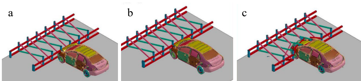
Fig. 6. Final frame for simulations at 50 km/h with different materials in the lateral protection systems: (a) S275; (b) Strenx 700 MC; (c) Aluminium 6005-T6
