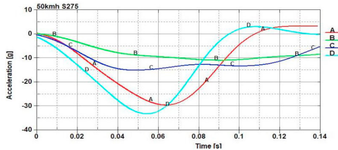
Fig. 5. Car deceleration (g's) for simulations at 50 km/h with S275 lateral protection systems: (A) Six-post system; (B) Two-post system; (C) Three-post system; (D) NCAP rigid wall
