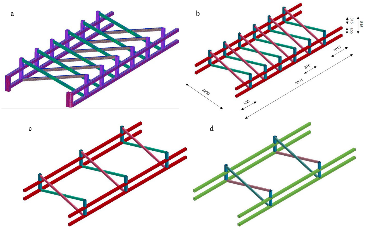
Fig. 1. (a) Six-post lateral protection system's FE model; (b) Main structural dimensions; (c) Three-post lateral protection system's FE model; (d) Two-post model lateral protection system's FE model
