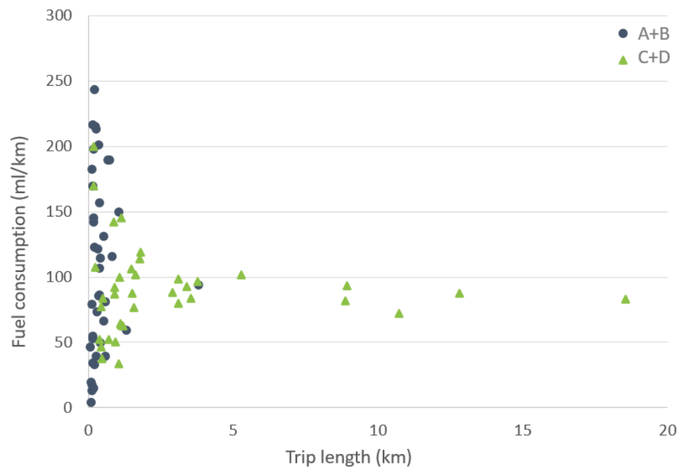
Figure 8. Comparison between fuel consumption for delivery micro-trips in the city center (A + B) or peri-urban (C + D) delivery area.
