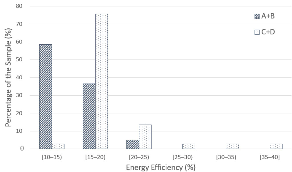
Figure 7. Comparison between energy efficiency proper for delivery micro-trips in the city center (A + B) or peri-urban (C + D) delivery area.
