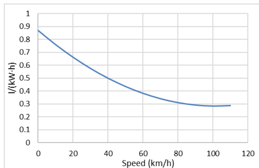
Figure 4. Fuel consumption/Energy ratio.
