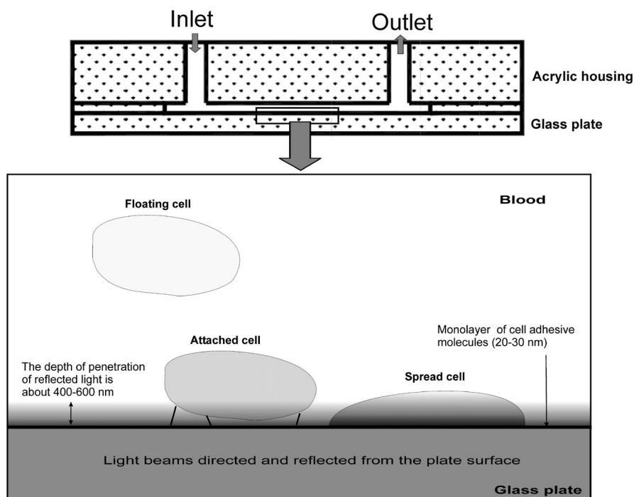
FIGURE 2 The illustration of the flow chamber with the flat glass surface coated with a monolayer of cell-adhesive molecules. The reflected light evanesces into the blood sample beyond the reflection zone to a depth of approximately 400–600 nm. Platelets or other blood cells in the flow do not interact with this laser radiation, which evanesces to such a small depth. The laser light can interact with platelets only when they are strongly attached to or spread onto the glass surface
