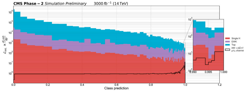
Fig. 4. Predictions of the classifier evaluated on the test dataset for the \mu\tau_h bb final state. Both signal and background are normalized to the expected yields. Images source [45] (supplementary material).
