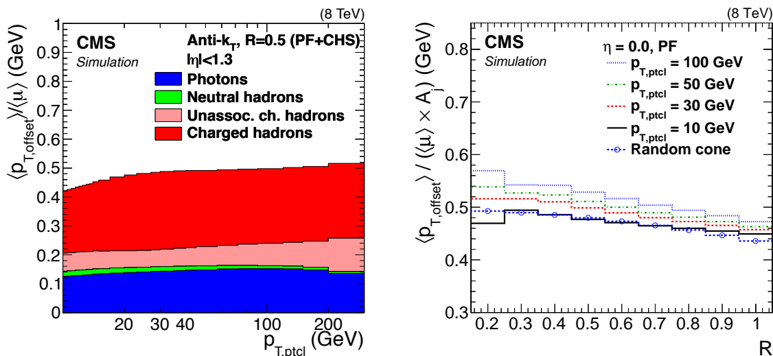
Figure 6. Simulated particle-level offset versus p_T separately for each type of PF candidate (left). Average p_T offset density versus jet distance parameter R for various p_{T,\text{ptcl}} compared to a random-cone offset density versus cone radius (right). The jet or cone area A_j corresponds to \pi R^2 .
