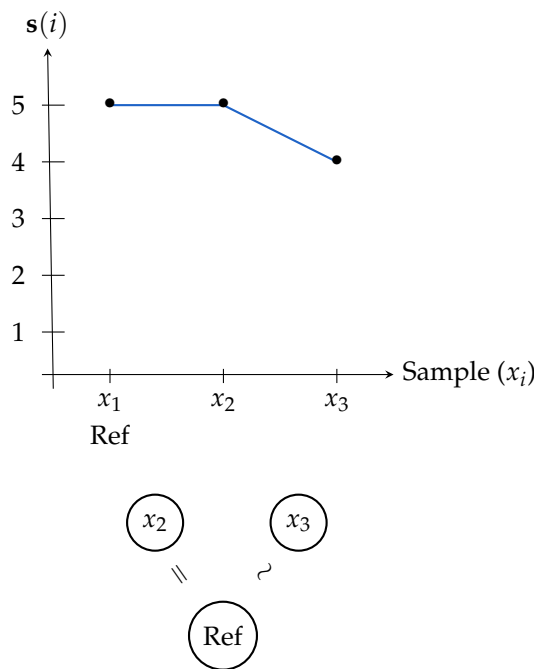
Figure 6. Example of scores describing that there is no significant difference between x_3 and the reference sample x_1 (equivalently, its identical to sample x_2 ) and where a threshold \epsilon = 1 is considered.
