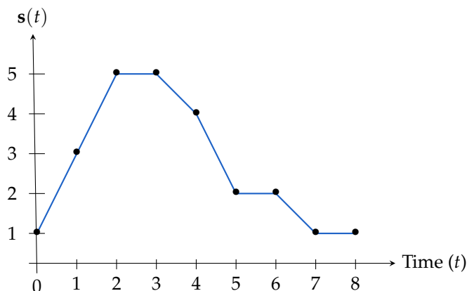
Figure 3. Example of scores describing the intensity of wine flavor showing a unimodal pattern.
