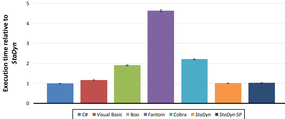
Figure 12: Execution times of fully type-annotated programs, relative to StaDyn .
