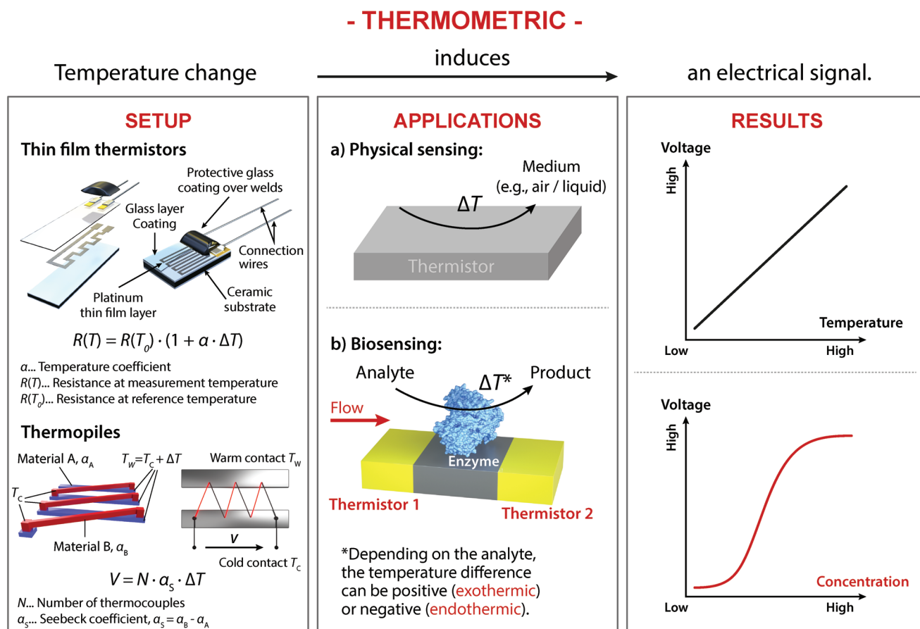
Figure 6. Thermometric signal transduction in disposable sensors. A temperature change caused by (a) the medium (such as gas or liquid) or (b) a target (bio)chemical substance (for example, a chemical reaction catalyzed by an enzyme for a certain substrate) produces an analytical (electrical) signal. Two notable examples are thin film thermistors (temperature-dependent resistors), and thermopiles. Thermopiles consist of a number of thermocouples, which generate a temperature-dependent voltage due to the thermoelectric effect (for example, Seebeck effect).
