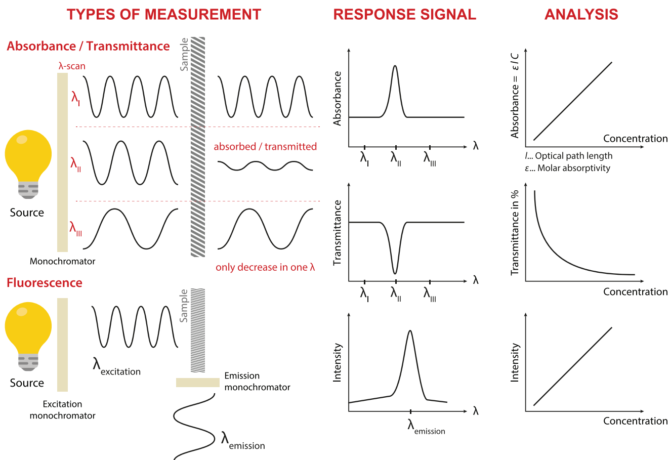
Figure 2. Optical signal transduction. Absorbance/transmission involves passing a beam of light (single or spectrum of wavelengths containing, for example \lambda_I , \lambda_{II} , and \lambda_{III} ) through the sample and measuring the amount of light absorbed or transmitted (here, \lambda_{II} ) on the opposite side using an optical detector. Note that in the illustration shown above, \lambda_I and \lambda_{III} do not interact with the sample; hence, the intensities of signals do not change. A monochromator can be used to scan ( \lambda -scan) a specific wavelength from the source. The amount of light absorbed or transmitted varies ( \lambda_{II} ) with the concentration of the analyte in the sample. Fluorescence involves excitation of a fluorescent compound with a beam of light. The excited molecule itself then emits light with an energy smaller than the energy of the source ( \lambda_{\text{emission}} < \lambda_{\text{excitation}} ). The intensity of the emitted light depends on the concentration of the fluorescent compound in the sample.
