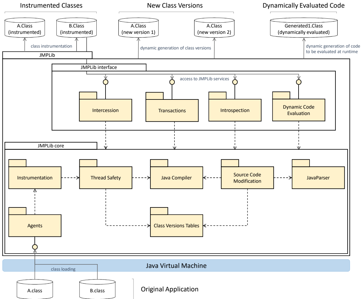
Figure 2: Architecture of JMPLib.
