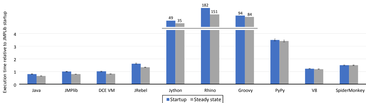
Figure 5: Average startup and steady-state execution times for 14 applications, relative to JMPLib startup.
