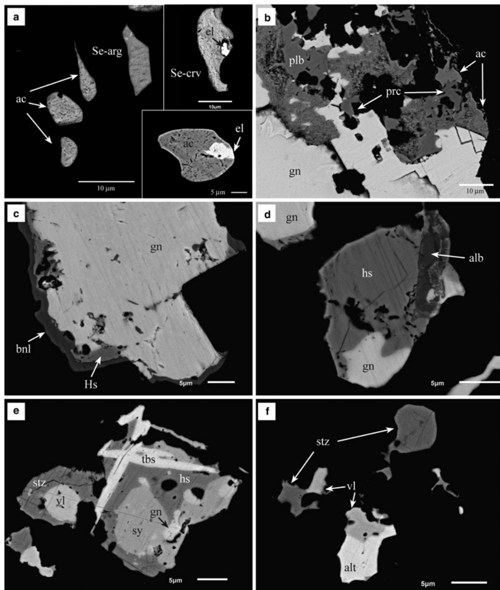
FIG. 7. Back-scattered electron images (BSE) of samples shown in Fig. 6. (a) Rounded and irregular inclusions of acanthite (ac), Se-bearing argyrodite (Se-arg) and Se-bearing cervelleite (Se-crv). Some inclusions contain minute grains of Au-Ag alloy (el). The BSE image, bottom right, is from sample DDH36-191; the others are from sample DDH31-79.5. (b) Detail of Fig. 6b. Galena has been partially replaced by pearceite (prc) and polybasite (plb), which are also replaced by acanthite (ac) with a porous, dusty appearance. (c) Galena surrounded by hessite (hs) and benleonardite (bnl). Sample DDH31-79.5. (d) A small grain of alburnite (alb) associated with hessite and galena. Sample DDH31-79.5. (e) Complex aggregate of tellurobismuthite (tbs), hessite (hs), stutzite (stz), sylvanite (sy), volynskite (vl) and galena (gn). Sample DDH33-203. (f) Irregular inclusions of tellurides in chalcopyrite including stutzite (stz), volynskite (vl) and altaite (alt) instead of galena. Sample DDH33-203.
