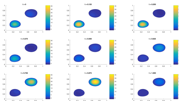
Fig. 2 Experiment 3. Support of the optimal 2D control at different moments of time. Piecewise constant functions. J_\sigma(\bar{u}_\sigma) = 0.01565574
