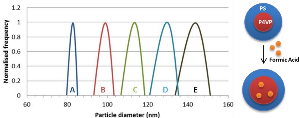
Figure 1. DLS size distributions for toluene solution of (PS- b -P4VP) (0.7 wt %) containing formic acid at different HCOOH/P4VP molar ratios: 0/1(A), 1/1 (B), 3/1 (C), 5/1 (D) and 10/1 (E) and schematic representation of micellar growth with the formic acid inclusion.
