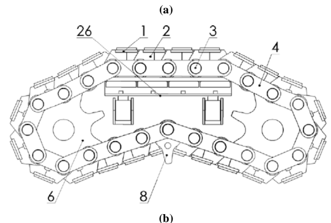
Fig. (2). Description of main elements.
