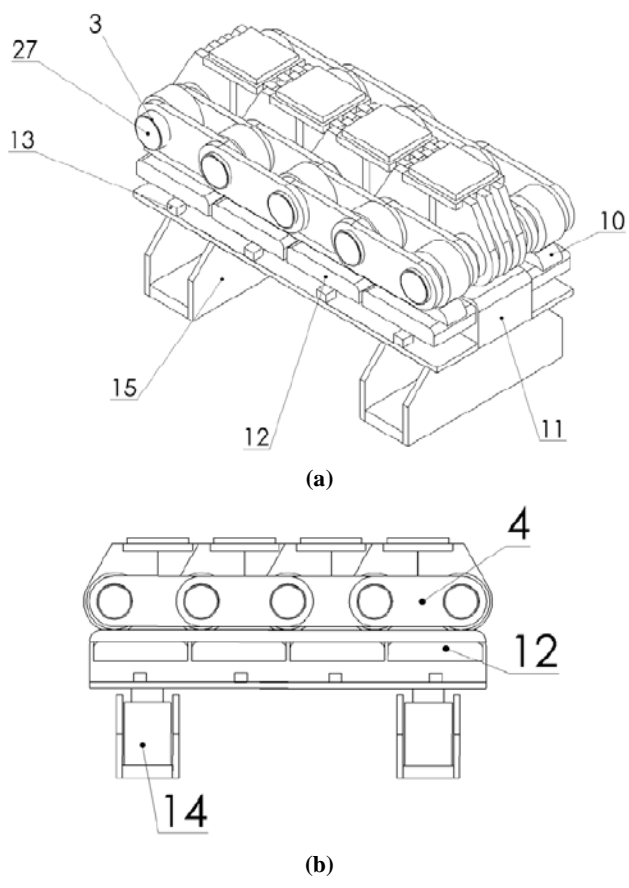
Fig. (4). Load compensation system of the launching mechanism.
