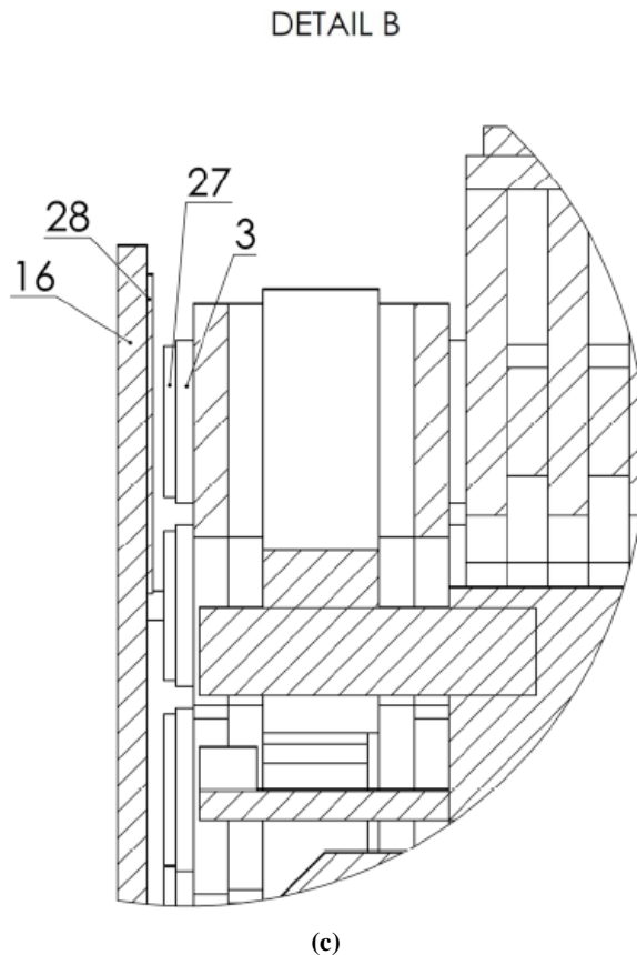
Fig. (5). Frictionless system: (a) Front view of the mechanism; (b) Section view of the mechanism; (c) Frictionless system details.
