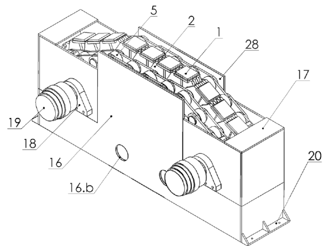
Fig. (1). Design of new mechanism to displace heavy structures.
