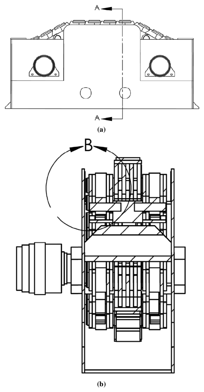
Fig. (3). Support links of the mechanism (2) and neoprene support sheets (1).
