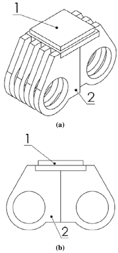
Fig. (3). Support links of the mechanism (2) and neoprene support sheets (1).
