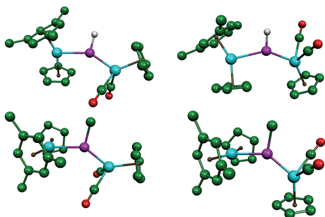
Fig. 2 DFT-optimized structures of the most stable isomers syn (left) and anti (right) of compounds 2 (above) and 3 (below), with most H atoms and ^1\text{Bu} groups (except their \text{C}^1 atoms) omitted for clarity.
