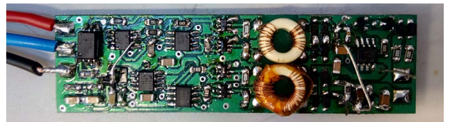
Fig. 8: Prototype of the gate driver (23.9x86.6 mm)
