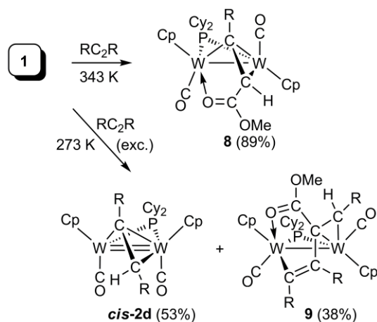
Scheme 3. Reactions of 1 with RC≡CR (R = CO 2 Me)
