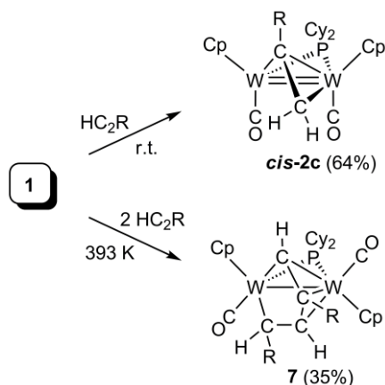
Scheme 2. Reactions of 1 with HC≡CR (R = CO 2 Me)
