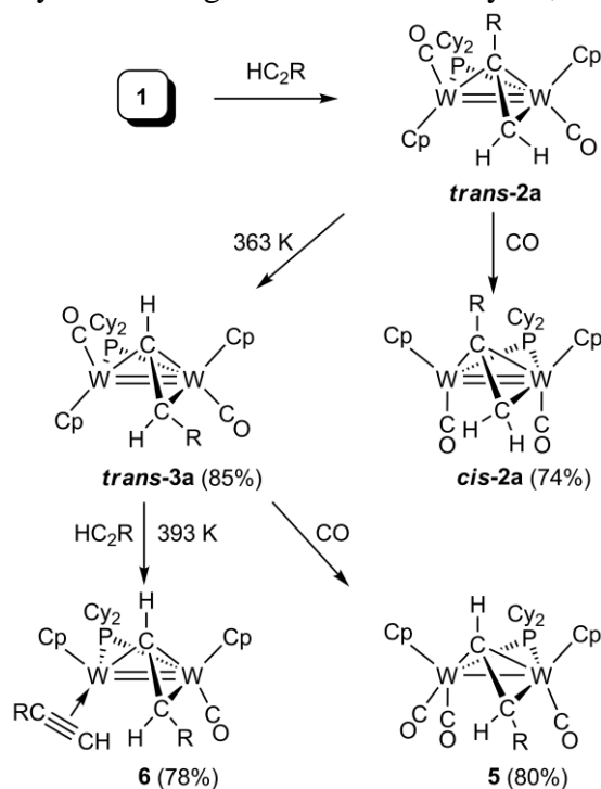
Scheme 1. Reactions of 1 with \text{HC}\equiv\text{CR} ( \text{R} = p\text{-tol} )
