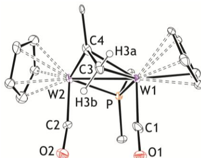
Figure 2. ORTEP diagram (30% probability) of compound cis-2a with H atoms (except H3a and H3b) and p -tol and Cy groups (except their C 1 atoms) omitted for clarity.
