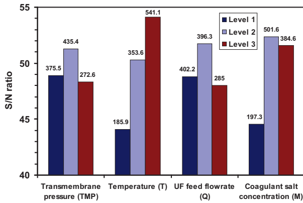
Fig. 5. Variation of permeate flux ( \text{L m}^{-2} \text{h}^{-1} ) and S/N ratio for different factors.
