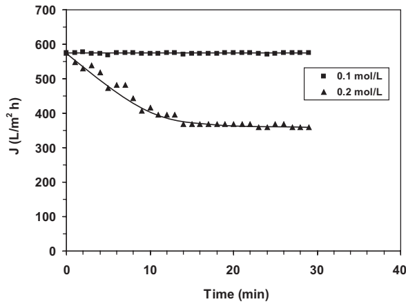
Fig. 4. Effect of coagulant salt concentration on permeate flux reduction for UF of \text{CaCl}_2 aqueous solutions. Operating conditions: Q = 90 \text{ L h}^{-1} , \text{TMP} = 2 \text{ bar} , and T = 20^\circ\text{C} .
