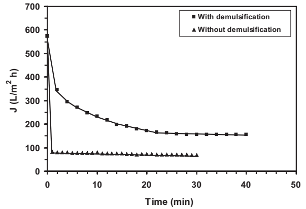
Fig. 2. Permeate flux reduction for UF of the fresh O/W emulsion and the centrifuged aqueous phase obtained after O/W emulsion demulsification with 0.1 \text{ mol L}^{-1} \text{CaCl}_2 . Operating conditions: Q = 90 \text{ L h}^{-1} , \text{TMP} = 2 \text{ bar} , and T = 20^{\circ}\text{C} .
