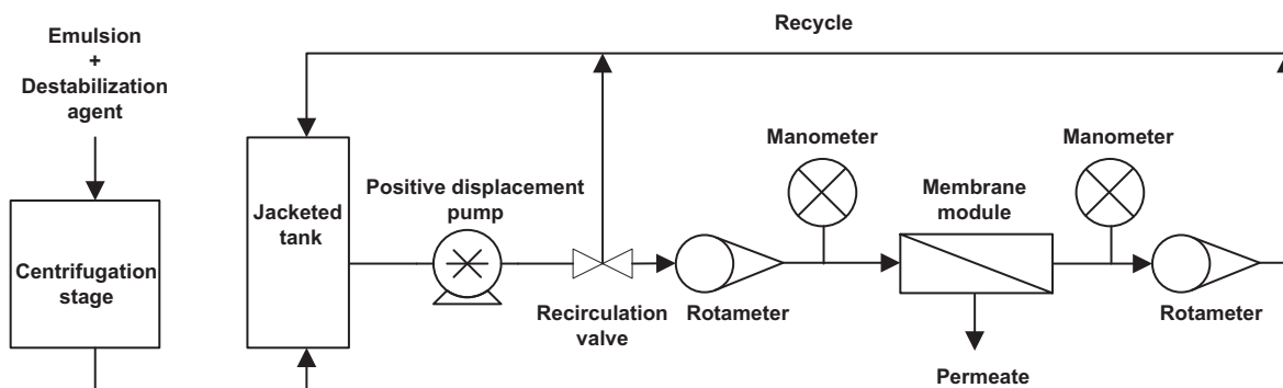
Fig. 1. Schematic diagram of the membrane hybrid process.
