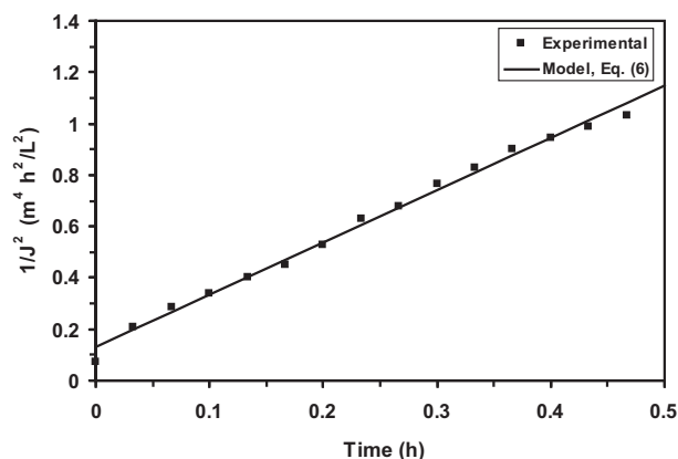
Fig. 3. Permeate flux predicted by the cake/gel layer formation model for the UF of the centrifuged aqueous phase obtained after O/W emulsion demulsification with 0.1 \text{ mol L}^{-1} \text{CaCl}_2 . Operating conditions: Q = 90 \text{ L h}^{-1} , \text{TMP} = 2 \text{ bar} , and T = 20^\circ\text{C} .
