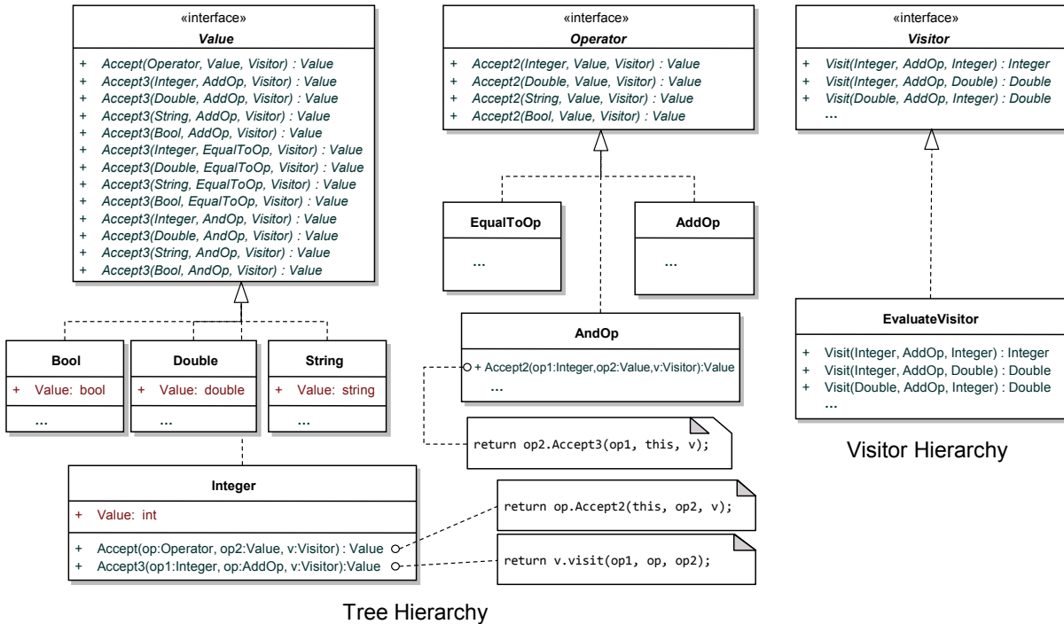
Figure 2. Multiple dispatch implementation with the statically typed approach (ellipsis obviates repeated members). Source: The authors
