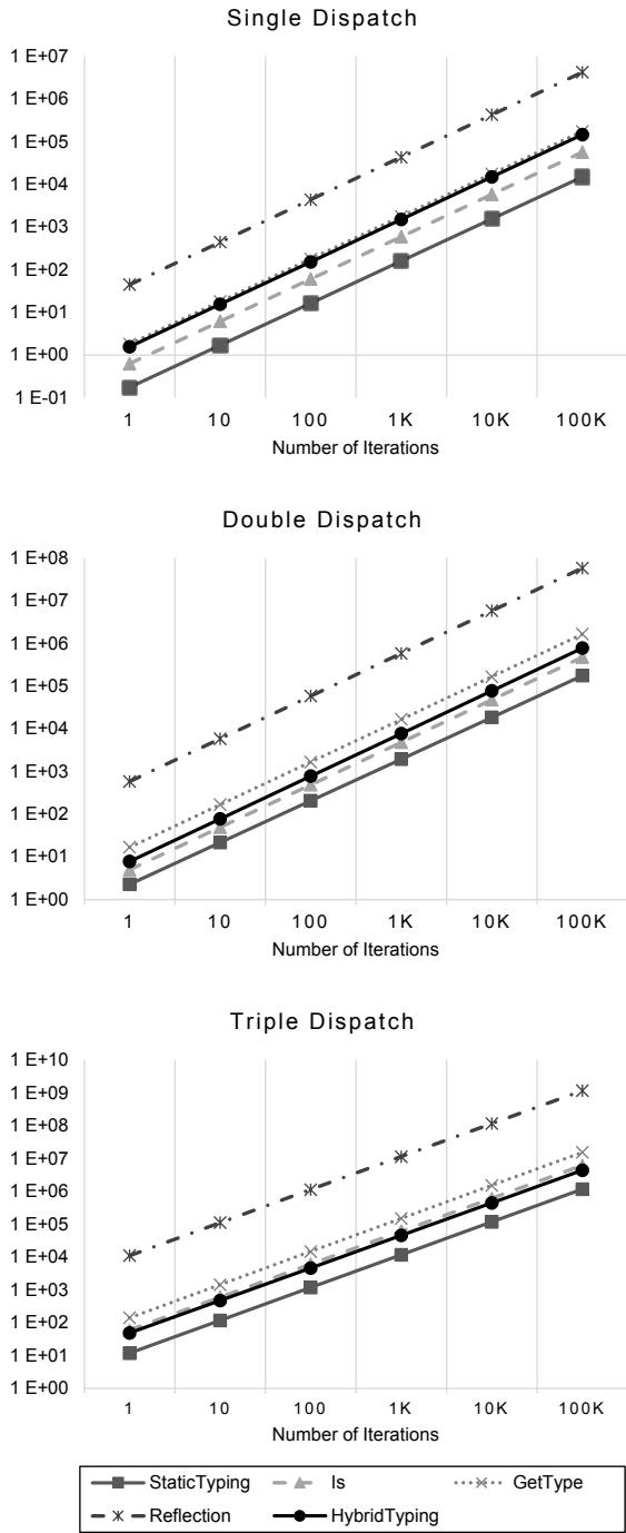
Figure 6. Execution time (microseconds in logarithmic scale) increasing the number of iterations. Source: The authors
