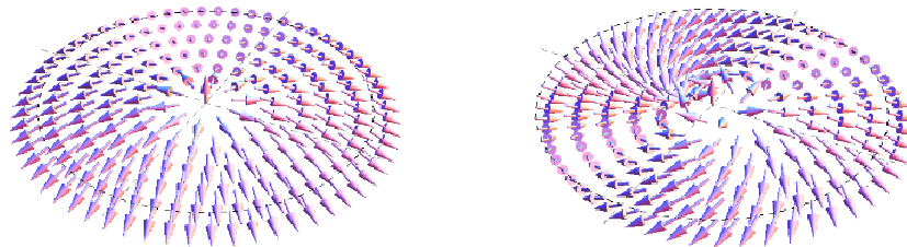
Figure 5. Graphical representation of the isospin vortex field \Phi = (\Phi_1(x_1, x_2), \Phi_2(x_1, x_2), \Phi_3(x_1, x_2)) for the \psi -vortices with n = 1 (left) and n = 2 (right) for a = 1 in the spatial plane.
