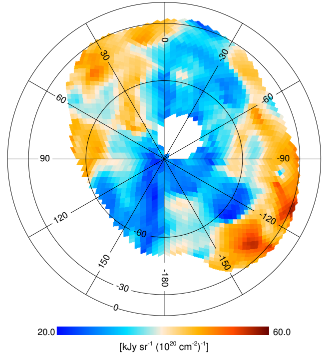
Fig. 3. Map of the dust emissivity at 353 GHz, i.e. the correlation measure \alpha_{353} with the CMB contribution \alpha(C_{\text{HI}}) subtracted [see Eq. (6)]. The correlation measure is computed in each pixel correlating the Planck map with the H I template over a sky patch with 15° diameter centred on it.
