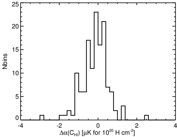
Fig. B.1. Histogram of the difference between two estimates of \alpha(C_{\text{HI}}) (the correlation measure between the CMB and the H I template), found assuming a greybody spectrum for the dust emissivity or calculated with the SMICA CMB map. The standard deviation of the difference, 0.7 \mu\text{K per } 10^{20} \text{ H cm}^{-2} , is 3% of the standard deviation of \alpha(C_{\text{HI}}) .
