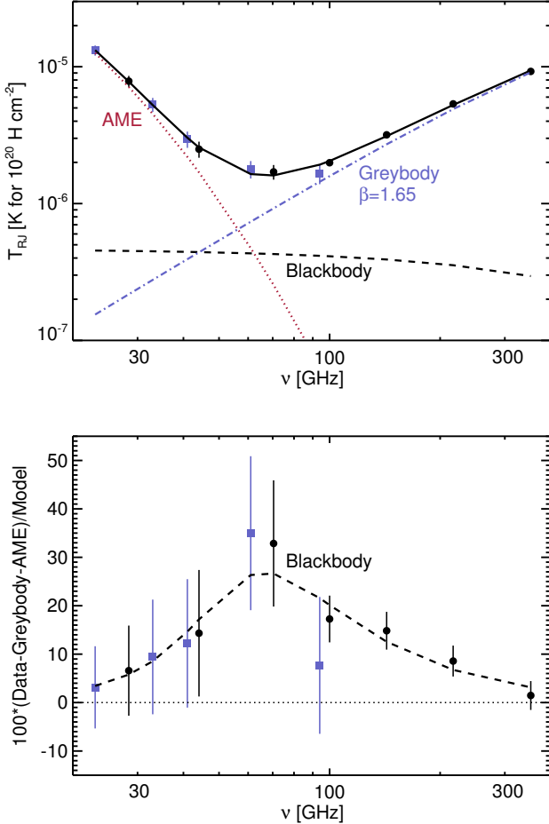
Fig. 16. Top: Same microwave dust SED as in Fig. 15 with the spectral fit for model 2 in Table 4. The spectral index of the greybody is fixed to the value \beta_{\text{FIR}} = 1.65 inferred from the fit of the dust SED at \nu \geq 353 GHz (Table 3). The AME is fitted with the analytical model in Eq. (10). This fit includes a third component represented by a blackbody spectrum at the same temperature (19.8 K) as that of the greybody. Bottom: Blackbody component in model 2 as a fractional residual after subtraction of the AME and greybody emission from the total, compared to the data residuals.
