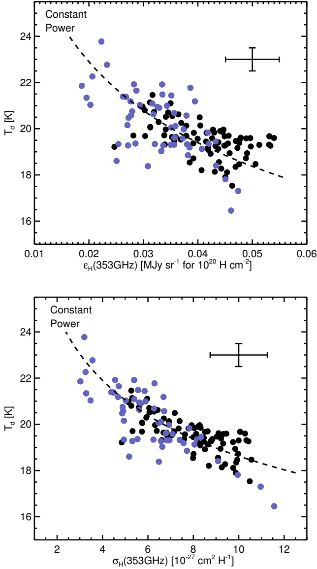
Fig. 9. Top: Dust colour temperature T_d versus dust emissivity at 353 GHz, two independent observables (Fig. 3), with typical error bars at the top right. The dashed line represents the expected dependency of T_d on the dust emissivity for a fixed emitted power of 3.4 \times 10^{-31} \text{ W H}^{-1} . The blue dots identify data for sky patches centred at Galactic latitudes b \leq -60^\circ . Bottom: T_d versus dust opacity at 353 GHz, re-expressing the same data in the form plotted by Planck Collaboration XXIV (2011) and Martin et al. (2012).
