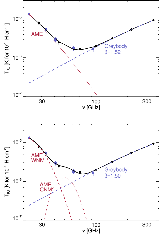
Fig. 15. Mean microwave dust SED obtained by cross-correlating the Planck and WMAP data with the H I and 408 MHz templates (black dots for Planck and blue squares for WMAP ). Top : Model 1 in Table 4, with two emission components combining AME and greybody thermal dust emission with \beta = 1.52 . The AME is fitted with the analytical model in Eq. (10). Bottom : Spectral fit for model 3, where the AME is fitted with two SPDUST spectra peaking at different frequencies.
