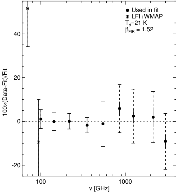
Fig. 13. Top: Residuals from a greybody fit of the mean dust SED at \nu \geq 353 GHz, using one spectral index. Dashed error bars are the quadratic sum of the statistical error (solid) and the photometric uncertainty. The photometric uncertainty is dominant at \nu \geq 545 GHz and negligible for the lower frequencies. Bottom: Residuals from a greybody fit to all data points down to 100 GHz, again using a single spectral index.
