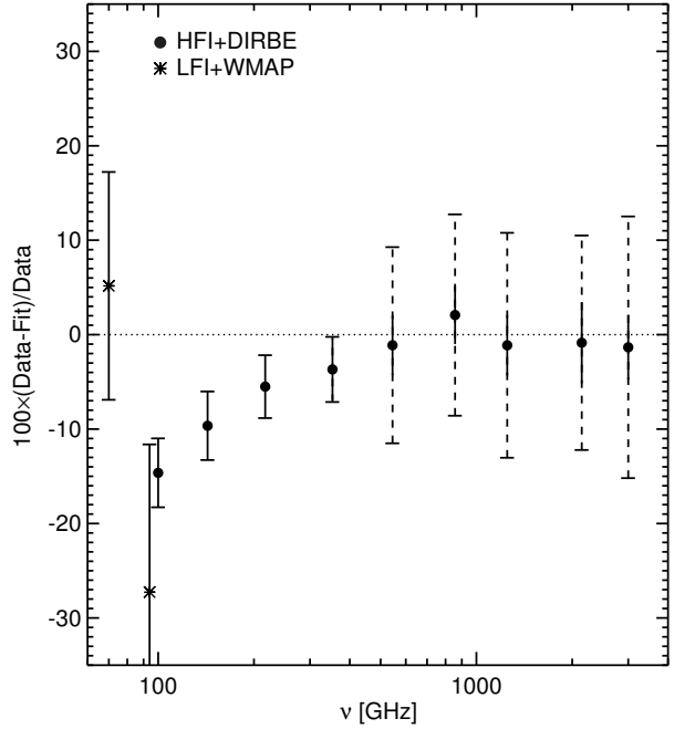
Fig. 14. Same as Fig. 13, but for residuals from fits of the mean dust SED with the DUSTEM (top panel) and DL07 (bottom panel) dust models.
