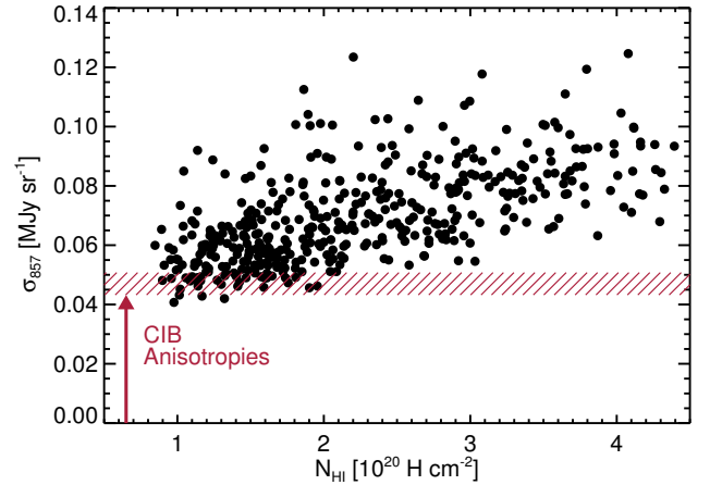
Fig. 7. Standard deviation \sigma_{857} of the residuals with respect to the Planck -H I correlation at 857 GHz versus the mean N_{\text{HI}} , both computed within circular sky patches with 5^\circ diameter and over unmasked pixels. The red hatched strip marks the contribution of CIB anisotropies to the residuals at 16' resolution, computed from the CIB model in Planck Collaboration XXX (2014). The width of the strip represents the expected scatter ( \pm 1 \sigma ) of this contribution. Both the scattered distribution of data points above CIB anisotropies strip and the increase in the mean \sigma_{857} with N_{\text{HI}} arise from residuals with a Galactic origin (Appendix D).
