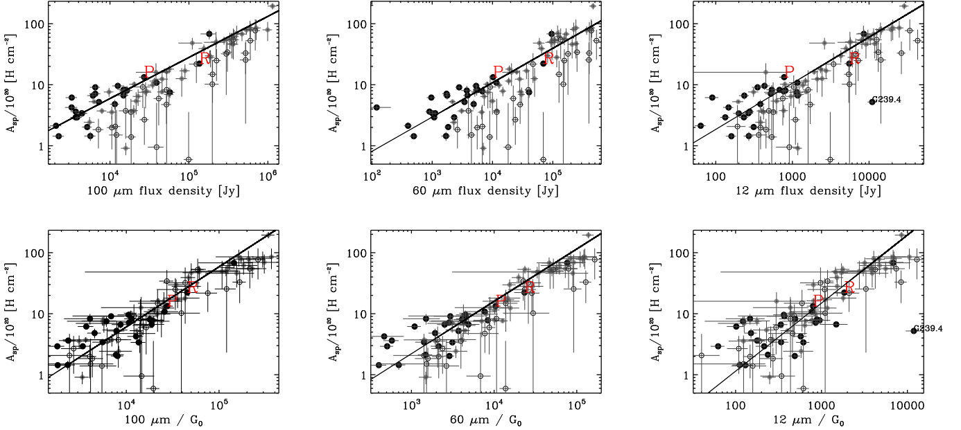
Fig. 18. Top row: AME amplitude ( A_{\text{sp}} ) as a function of the 100\ \mu\text{m} ( left ), 60\ \mu\text{m} ( middle ), and 12\ \mu\text{m} ( right ) flux density. Bottom row: The same as the top row, except that the FIR flux densities have been divided by G_0 . Symbols are as in Fig. 6. The best-fitting slope fitted to the significant AME regions only is plotted. The Perseus (P) and \rho Ophiuchi (R) clouds are indicated. There is a strong correlation between the AME intensity and infrared tracers of dust, with an improved correlation after dividing by G_0 . At 12\ \mu\text{m} the fit is made excluding the outlier source G239.40–4.70 (marked).
