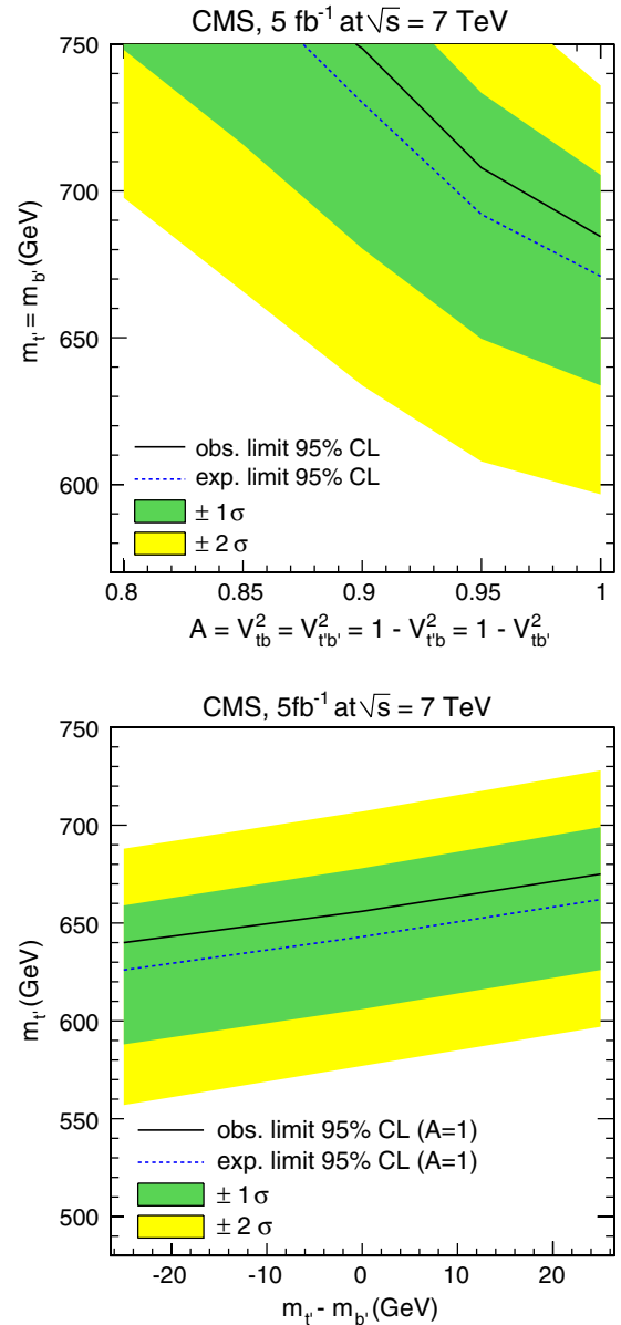
FIG. 2 (color online). Top: Exclusion limit on m_{t'} = m_{b'} as a function of the V_{\text{CKM}}^{4 \times 4} parameter A . The parameter values below the solid line are excluded at 95% CL. The inner (outer) band indicates the 68% (95%) confidence interval around the expected limit. The slope indicates the sensitivity of the analysis to the t'b and tb' processes. Bottom: For a V_{\text{CKM}}^{4 \times 4} parameter value A \sim 1 , the exclusion limit on m_{t'} versus m_{t'} - m_{b'} is shown. The exclusion limit is calculated for mass differences up to 25 GeV. The existence of up-type fourth-generation quarks with mass values below the observed limit are excluded at the 95% CL.
