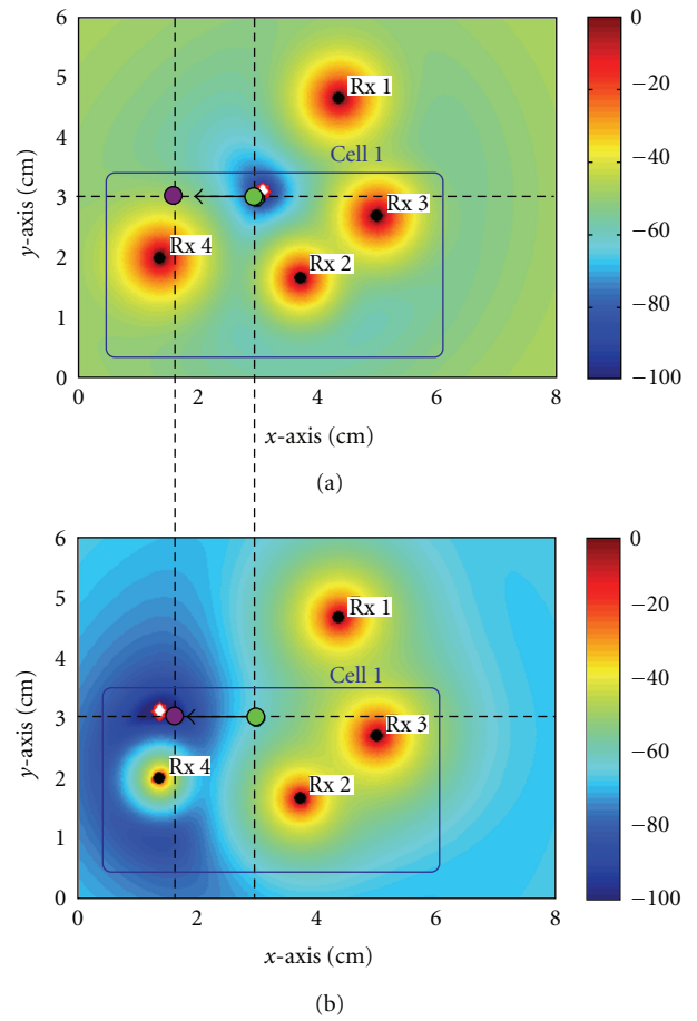
FIGURE 15: Location method evaluation in Positions 1(a) and 2(b) using RSS measurements from ZigBee nodes. Colormap represents the cost function evaluation at each point of the scenario.
