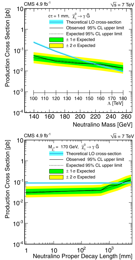
Fig. 7. Upper limits at the 95% CL on the cross section as a function of the \tilde{\chi}_1^0 mass for c\tau = 1 mm (top), and for the \tilde{\chi}_1^0 proper decay length for M_{\tilde{\chi}_1^0} = 170 GeV (bottom) in the SPS8 model of GMSB supersymmetry. (For interpretation of the references to color in this figure legend, the reader is referred to the web version of this Letter.)
