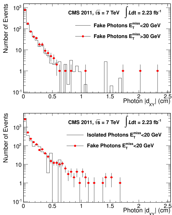
Figure 4. Top: fake photon |d_{XY}| distributions in the background ( E_T^{\text{miss}} < 20 GeV) and signal ( E_T^{\text{miss}} > 30 GeV) regions. Bottom: isolated and fake photon |d_{XY}| distributions in the background region ( E_T^{\text{miss}} < 20 GeV).
