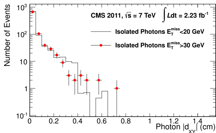
Figure 5. |d_{XY}| distributions for isolated photons: background region ( E_T^{\text{miss}} < 20 GeV) compared to the signal region ( E_T^{\text{miss}} > 30 GeV).
