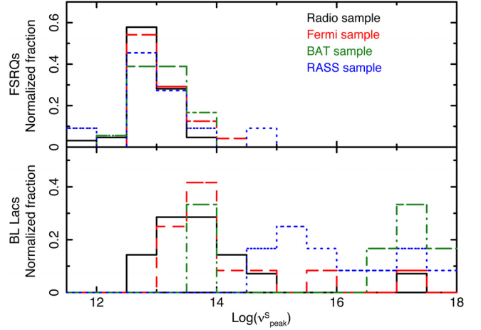
Fig. 17. The rest-frame synchrotron \nu_{\text{peak}}^{\text{S}} distributions of FSRQs and BL Lacs in different samples. Black solid histograms: radio sample; red dashed histograms: Fermi -LAT sample; green dot-dashed histograms: Swift BAT sample; blue dotted histograms: RASS sample.
