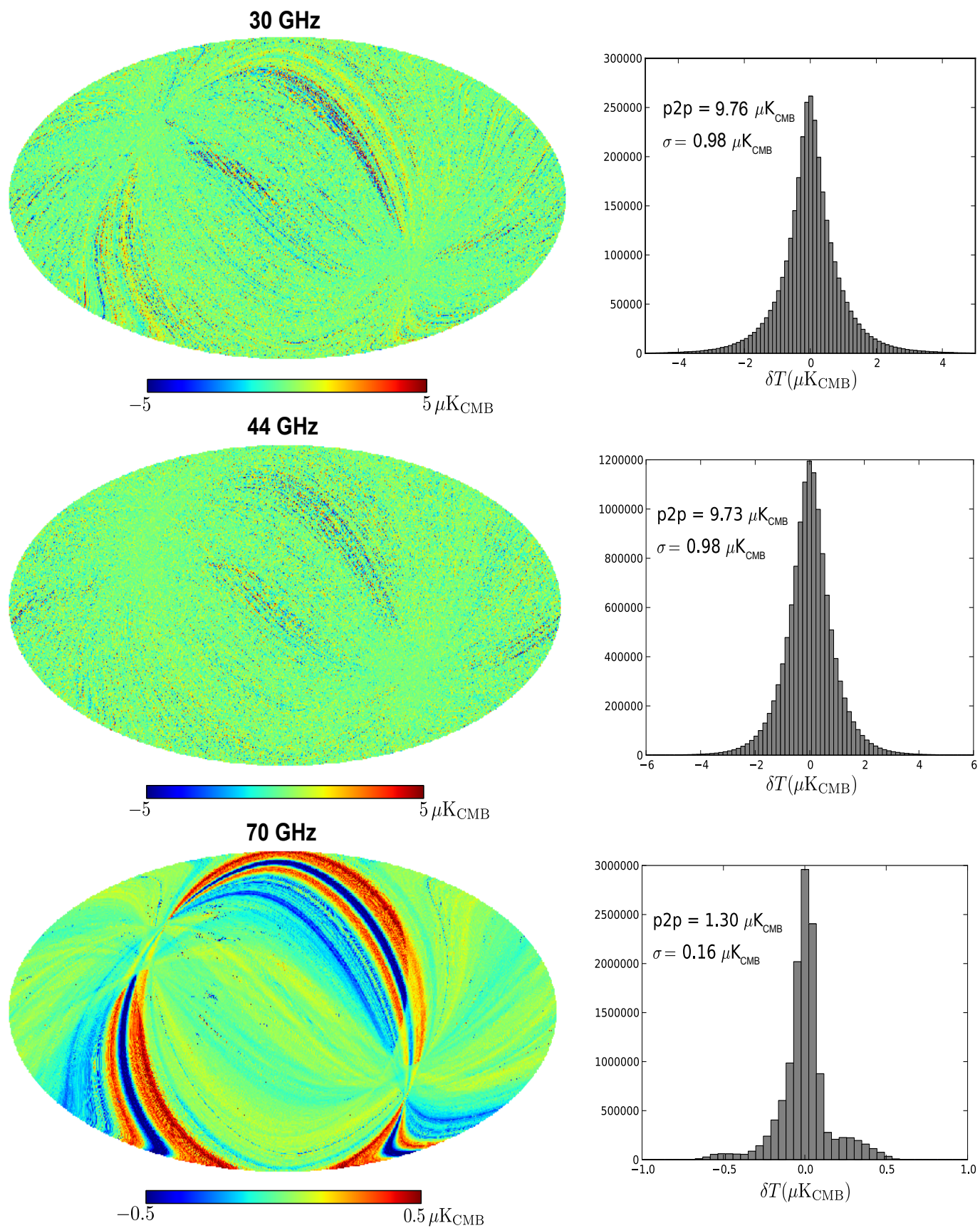
Fig. 31. Simulation of the systematic effects of temperature fluctuations of the 4 K reference loads. Maps are N_{\text{side}} = 512 at 30 GHz, and N_{\text{side}} = 1024 at 44 and 70 GHz. Note that the scale of 30 and 44 GHz maps is 10 times larger than then scale of the map at 70 GHz.
