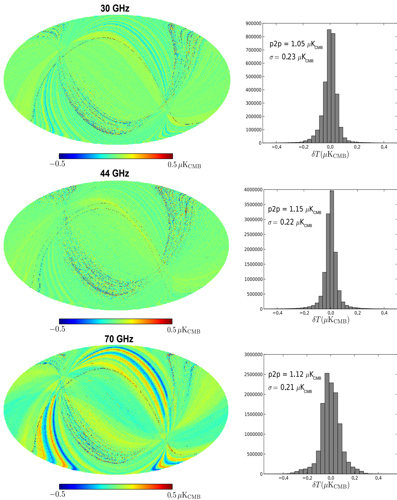
Fig. 30. Simulation of the systematic effects of temperature fluctuations of the LFI focal plane unit. Maps are N_{\text{side}} = 512 at 30 GHz, and N_{\text{side}} = 1024 at 44 and 70 GHz.
