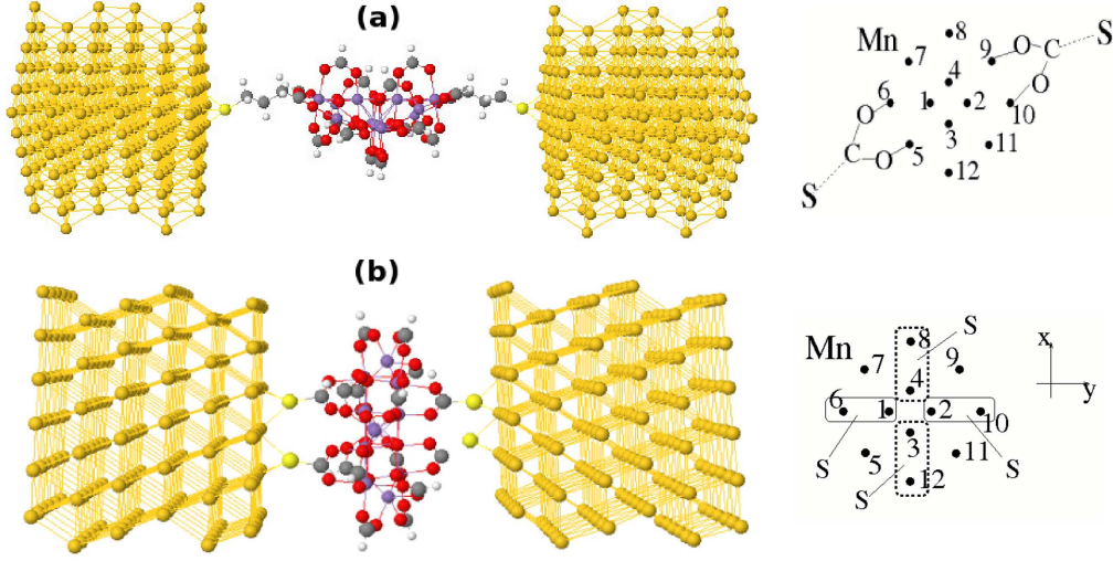
FIG. 1: (Color online) Scattering region for (a) geometry 1 consisting of \text{Mn}_{12} attached to Au layers via S atoms and alkane chains (distance between the electrodes d= 25.7 \text{ \AA} ), and for (b) geometry 2 consisting of \text{Mn}_{12} , four S atoms, and Au layers ( d=14.5 \text{ \AA} ). The transport direction is along the horizontal axis, z axis. Semi-infinite Au electrodes are considered in calculations (not shown). On the right hand side the positions of the Mn ions are marked for each geometry. For geometry 1 the dashed lines indicate the alkane chains. For geometry 2 the solid and dashed blocks represent the areas where the four S atoms are attached through bonding to the C atoms.
