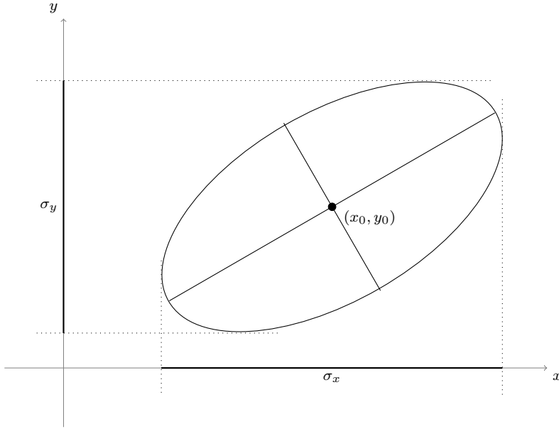
Fig. 1 The confidence ellipse for the nominal value (x_0, y_0) . The values \sigma_x, \sigma_y represent the marginal uncertainties of x_0, y_0 respectively, and depend on the value of \sigma .
