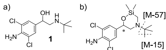
Figure 1 a) Clenbuterol. b) ^{13}\text{C}_1 -Labeled DMS-clenbuterol derivative and two of the characteristic breaks in its MS spectrum. The symbol * refers to the enriched ^{13}\text{C} position in the molecule
