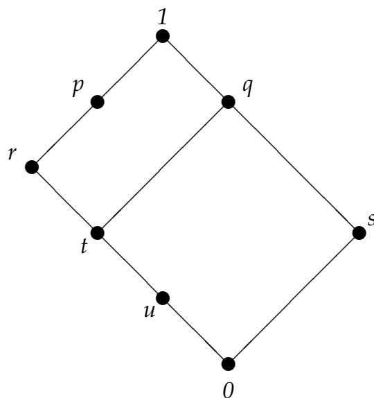
Figure 2. Lattice \Omega .
