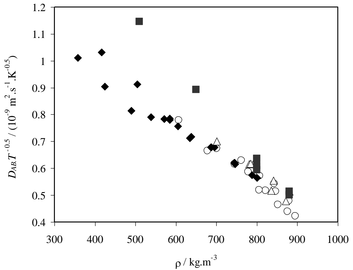
Figure 3. Values of D_{AB}/T^{0.5} as a function of density for mesitylene: \circ , this work; \triangle , Suarez et al. 1 ; \blacklozenge , Swaid and Schneider. 10 ; \blacksquare , Sassiat et al. 11
